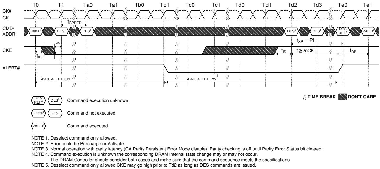
Figure 63. CA Parity Error Checking - PDE/PDX
