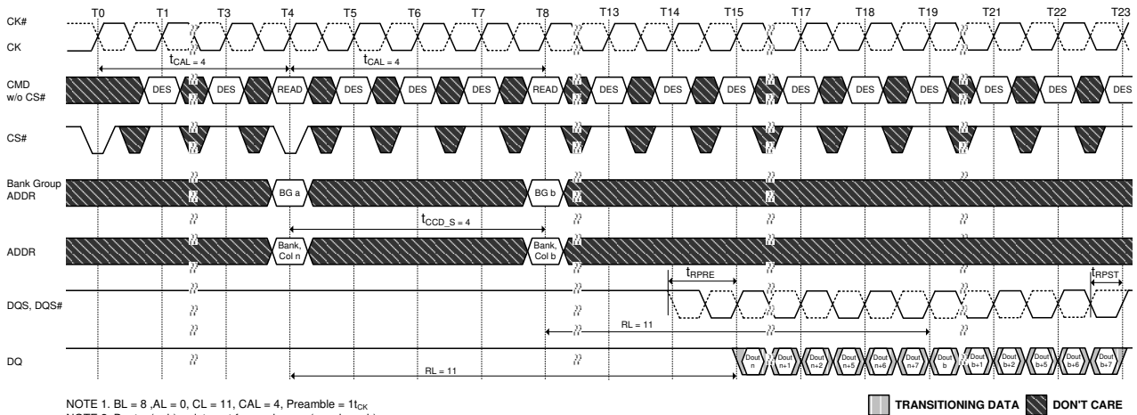
Figure 132. Consecutive Read (BL8) with CAL(4) and 1t CK Preamble in Different Bank Group
