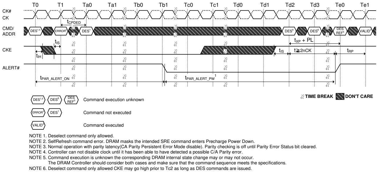
Figure 64. CA Parity Error Checking - SRE Attempt
