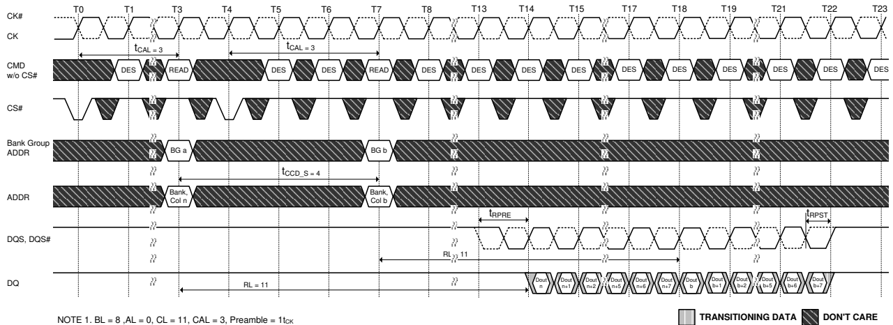
Figure 131. CAL consecutive Read (BL8) with CAL(3) and 1t CK Preamble in Different Bank Group
