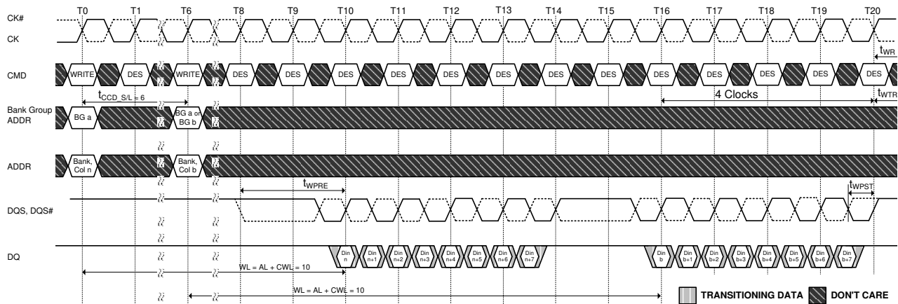
Figure 141. Nonconsecutive Write (BL8) with 1t_{CK} Preamble in Same or Different Bank Group
