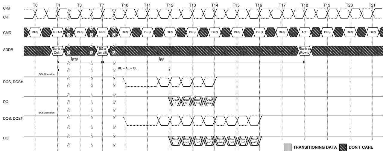
Figure 211. Read to Precharge with 1t_{CK} Preamble
