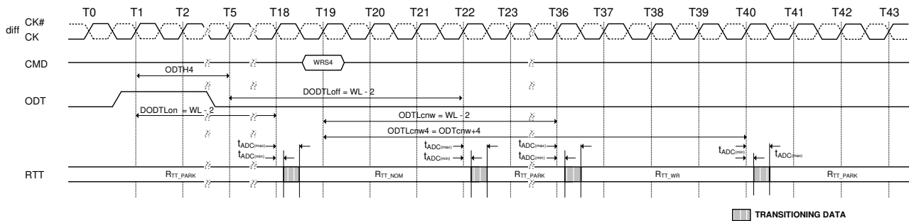
Figure 173. Synchronous ODT example with BL=4, CWL=9, AL=10, PL=0; DODTLon/off=WL-2=17, ODTcW=WL-2=17
