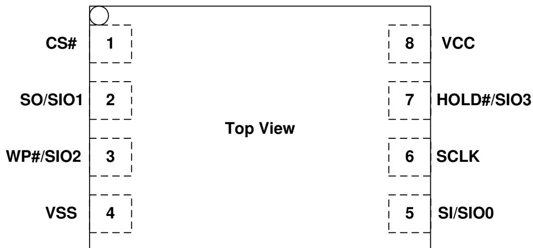
Figure 1-4. Pin Assignments
