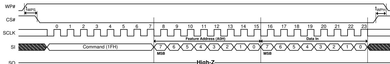
Figure 16-4. WP# Timing
