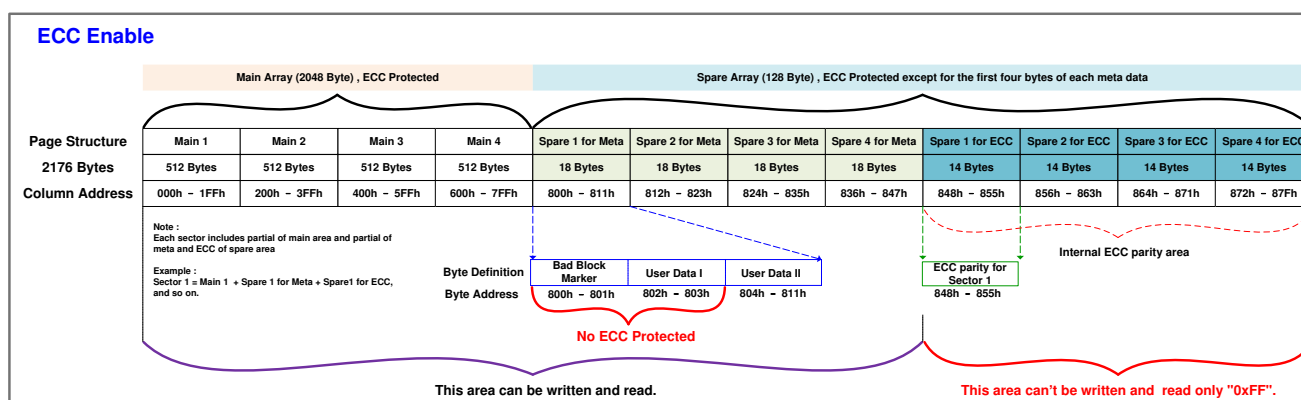
Figure 1-6. Architecture and Address of Page Size 2048+128 bytes
