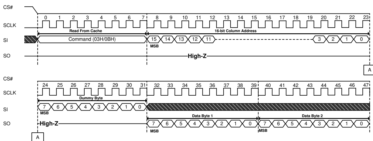
Figure 6-3. Read from Cache x1 IO (03H/0BH) Sequence Diagram
