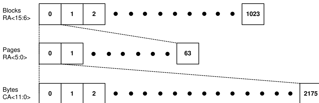
Figure 1-2. Memory Mapping Diagram for EM78C044VCG-H
