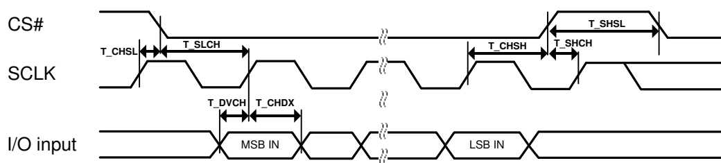
Figure 16-1. Serial Input Timing
