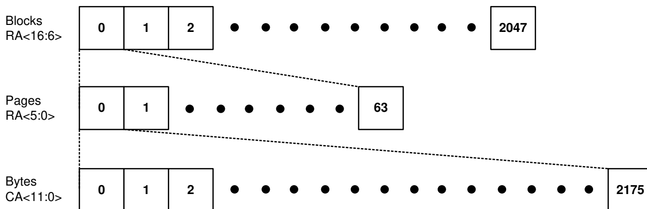
Figure 1-3. Memory Mapping Diagram for EM78D044VCG-H
