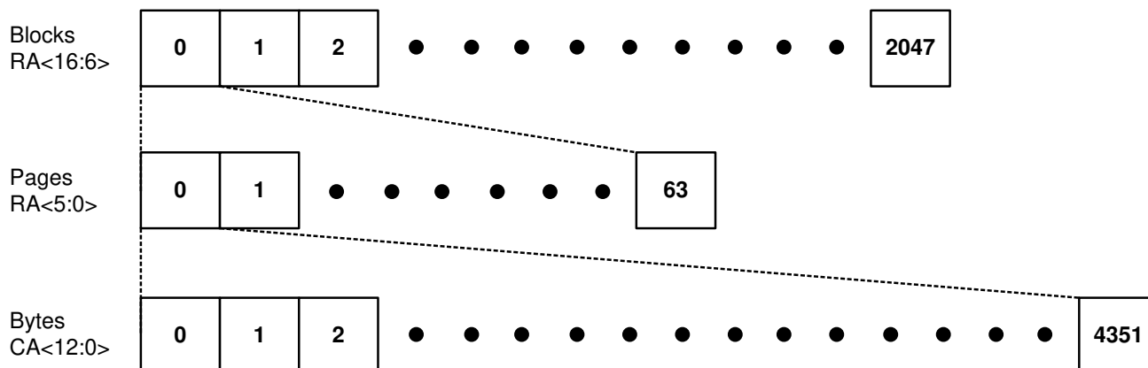
Figure 1-4. Memory Mapping Diagram for EM78E044VCE-H
