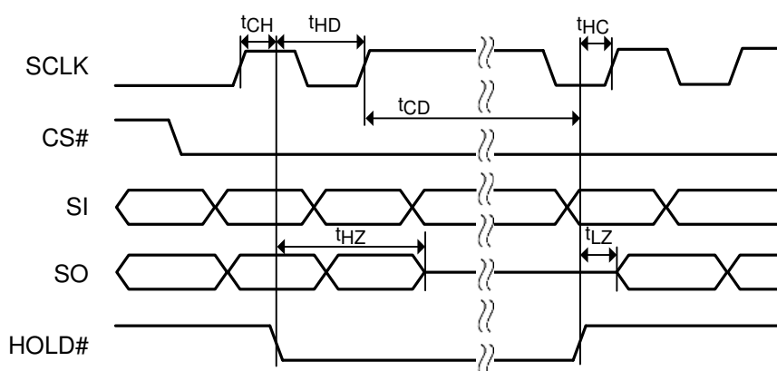
Figure 16-3. Hold# Timing
