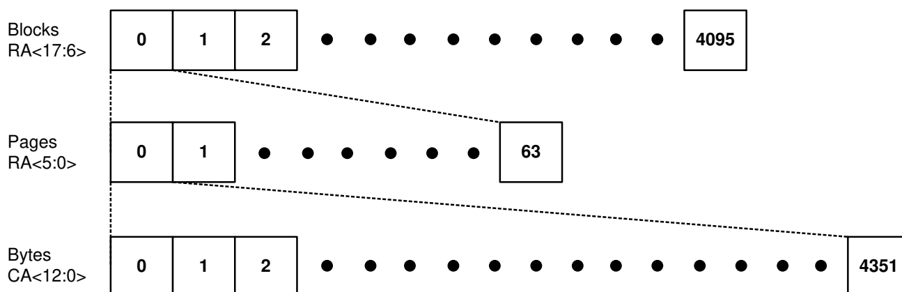
Figure 1-5. Memory Mapping Diagram for EM73F044VCE-H
