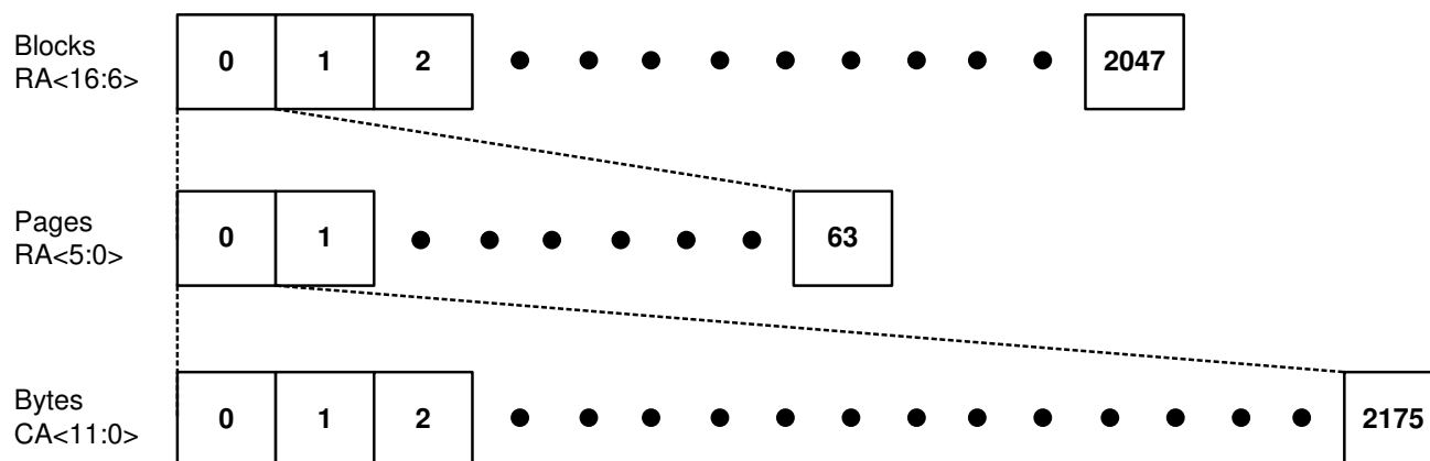
Figure 1-3. Memory Mapping Diagram for EM73D044VCU-H
