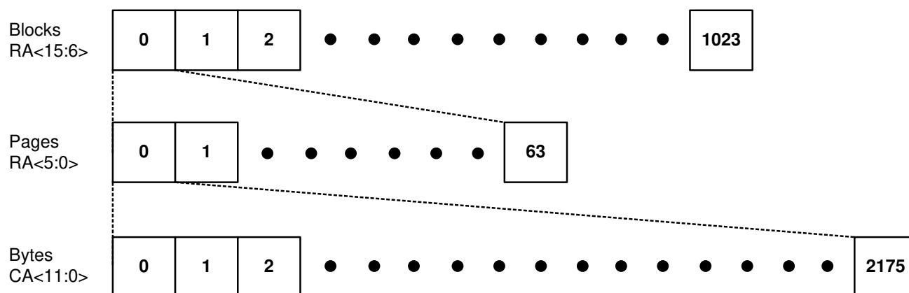
Figure 1-2. Memory Mapping Diagram for EM73C044VCH-H
