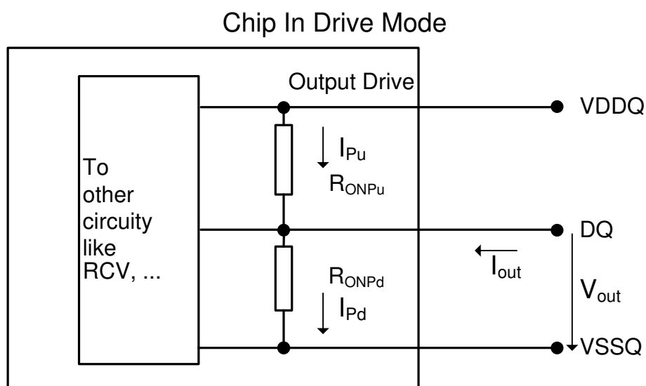
Figure 198. Output driver
