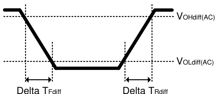
Figure 202. Differential Output Slew Rate Definition
