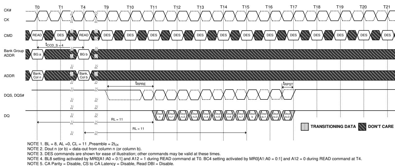
Figure 109. READ (BL8) to READ (BC4) OTF with 2t CK Preamble in Different Bank Group
