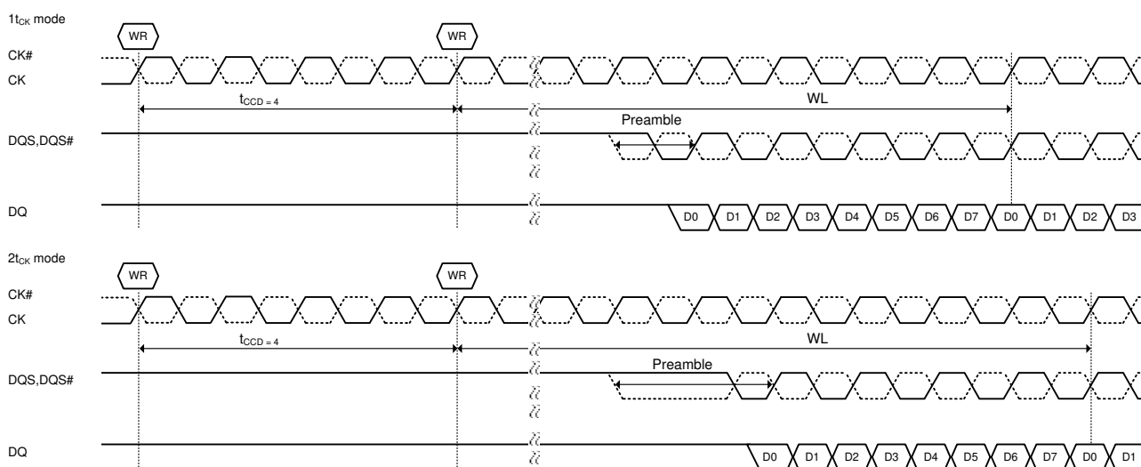
Figure 80. t_{CCD}=4 (AL=PL=0)
