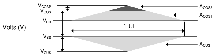
Figure 189. Clock Overshoot and Undershoot Definition
