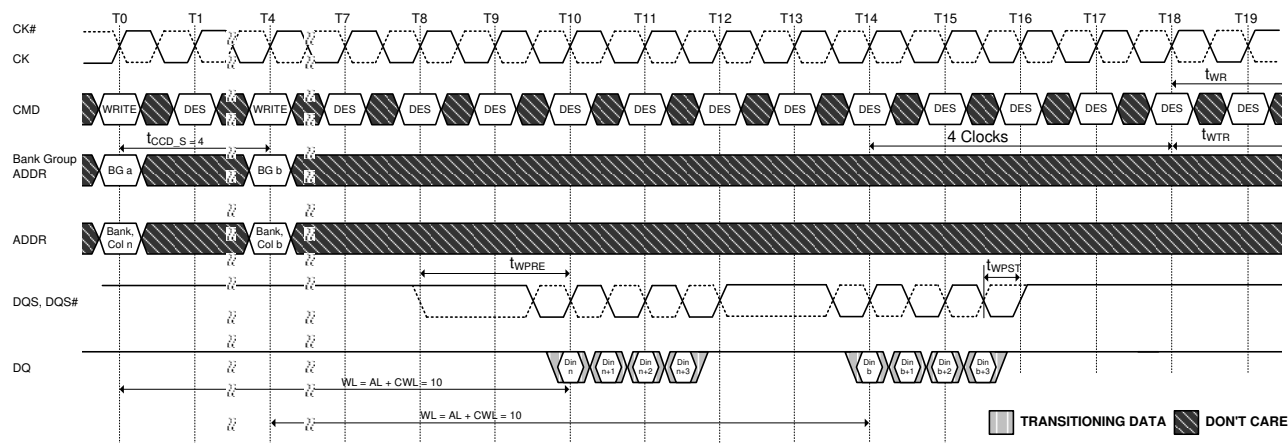
Figure 138. WRITE (BC4) OTF to WRITE (BC4) OTF with 1t CK Preamble in Different Bank Group
