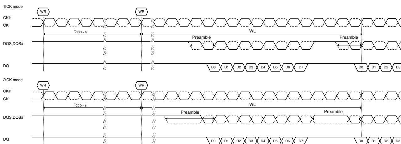
Figure 82. t CCD =6 (AL=PL=0)
