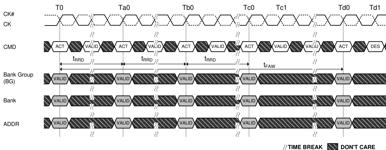
Figure 76. t FAW Timing
