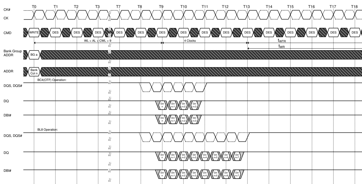
Figure 152. WRITE (BC4) Fixed with Auto PRECHARGE Operation and 1t_{CK} Preamble
