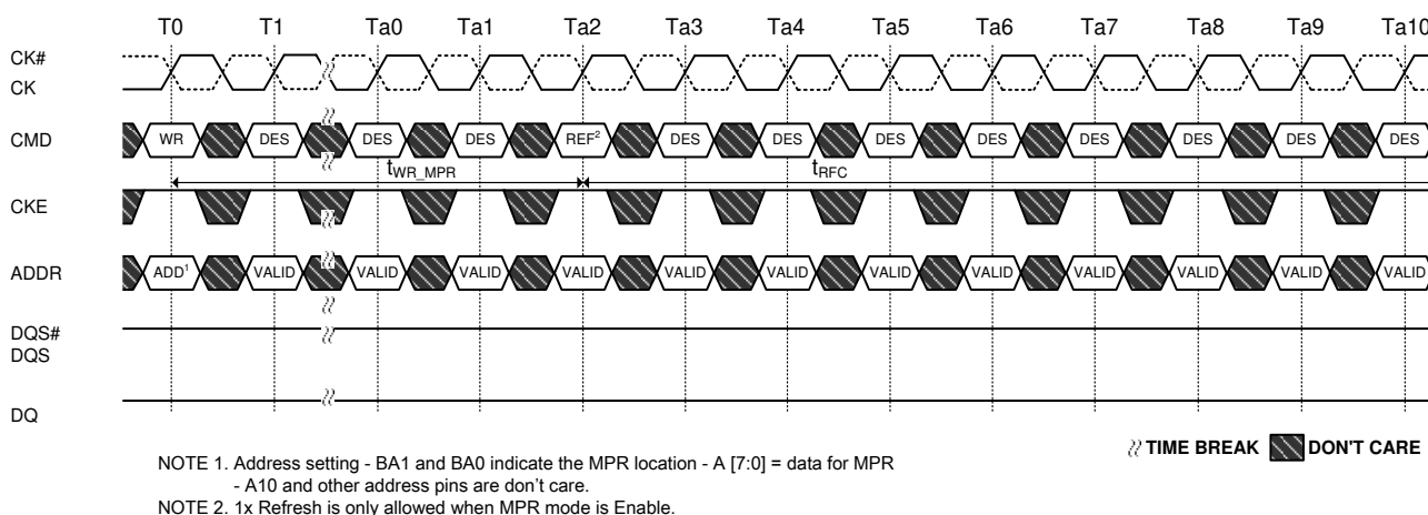
Figure 72. Write to Refresh Command Timing
