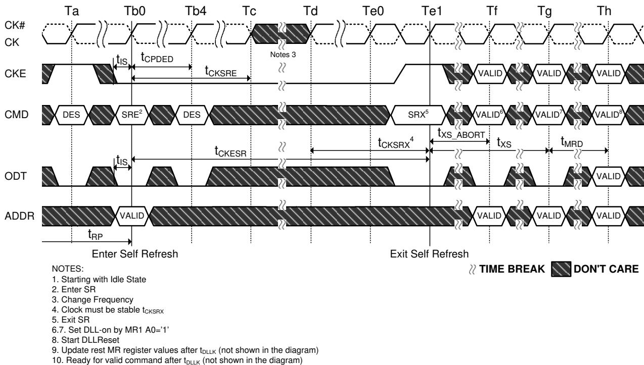
Figure 10. DLL Switch Sequence from DLL OFF to DLL ON
