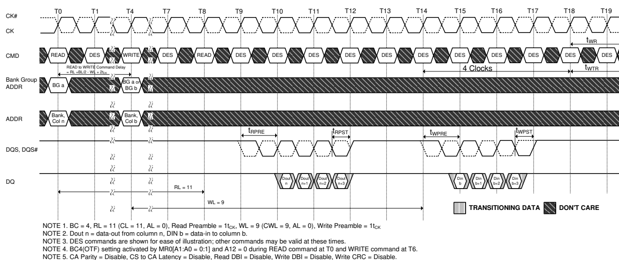
Figure 110. READ (BC4) to READ (BL8) OTF with 1t_{CK} Preamble in Different Bank Group
