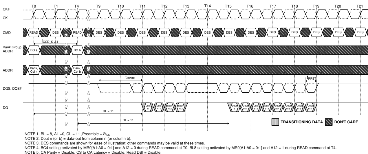
Figure 111. READ (BC4) to READ (BL8) OTF with 2t_{CK} Preamble in Different Bank Group
