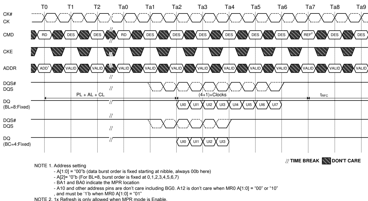
Figure 71. Read to Refresh Command Timing
