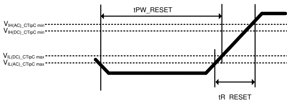
Figure 165. Input C Slew Rate Definition
