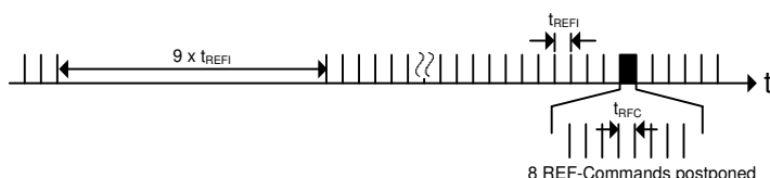
Figure 42. Postponing Refresh Commands (Example of 1X Refresh mode)
