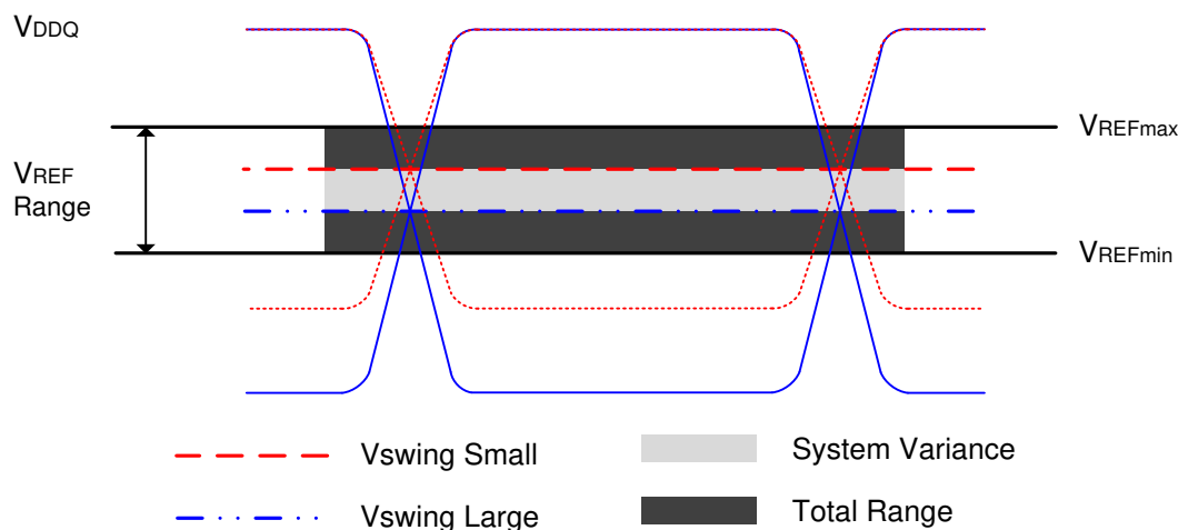
Figure 45. V REFDQ Operating Range (V REFmin , V REFmax )
