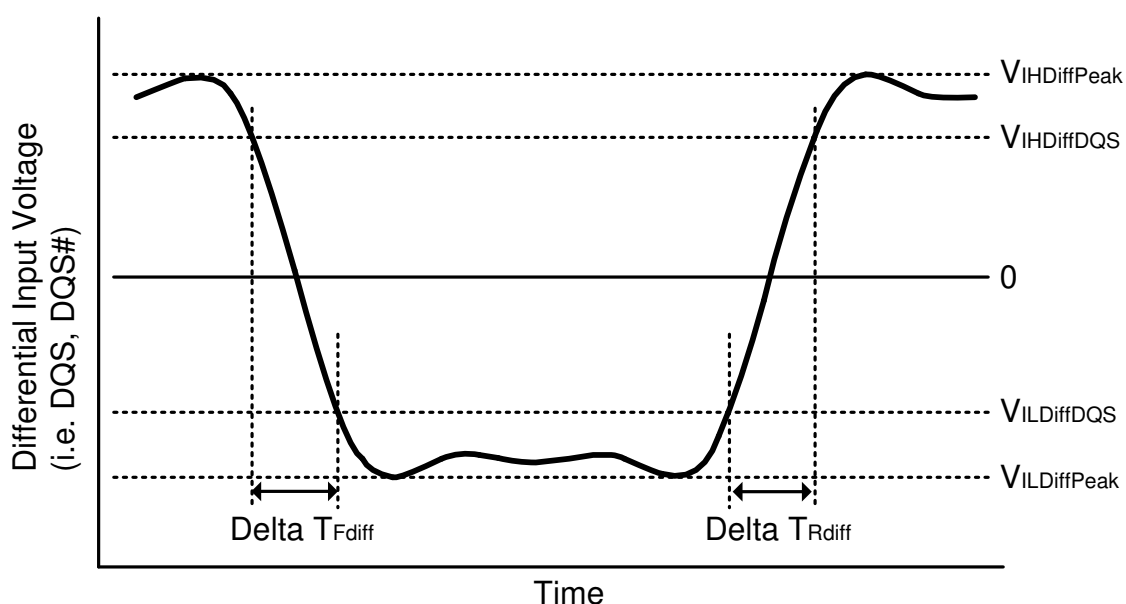
Figure 211. Differential Input Slew Rate Definition for DQS, DQS#
