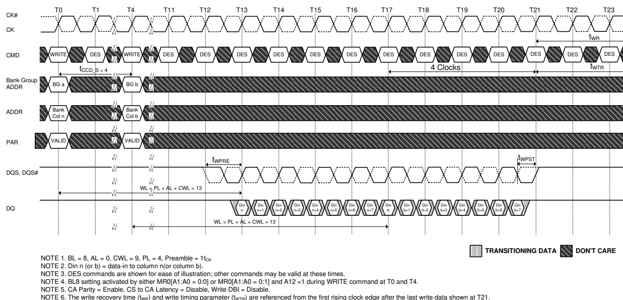
Figure 155. Consecutive WRITE (BL8) with 1t_{CK} Preamble and CA Parity in Different Bank Group
