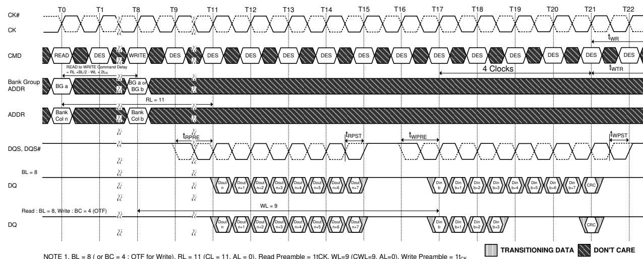
Figure 124. READ (BL8) to WRITE (BL8 or BC4: OTF) with 1t CK Preamble and Write CRC in Same or Different Bank Group
