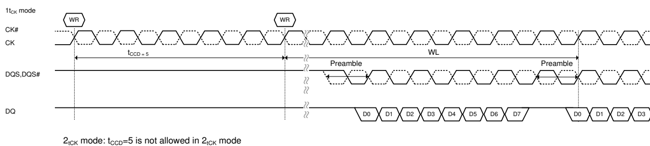
Figure 81. t CCD =5 (AL=PL=0)
