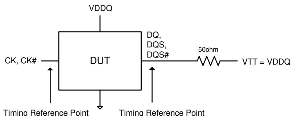
Figure 212. Reference Load for AC Timing and Output Slew Rate
