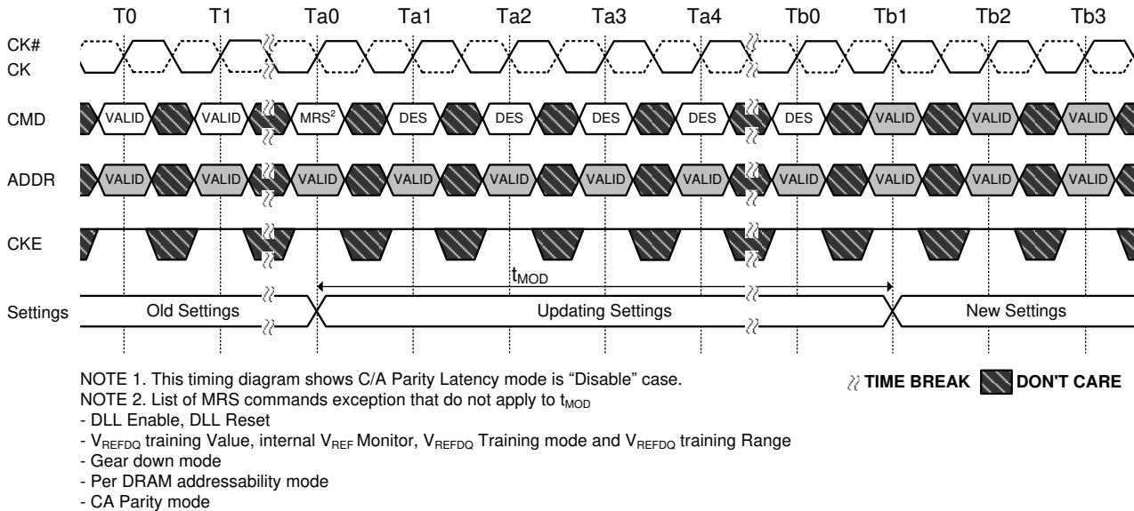
Figure 7. t_{MOD} timing
