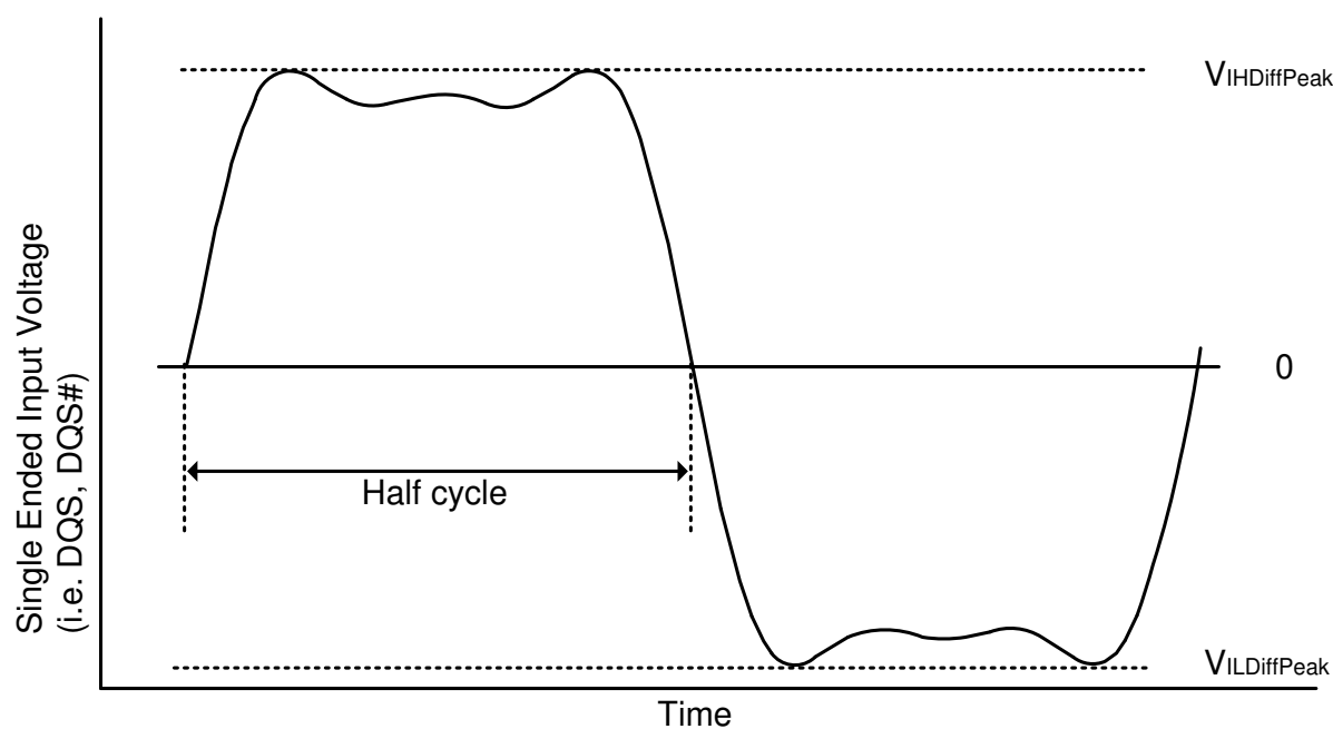
Figure 208. Definition of differential DQS Signal AC-swing Level
