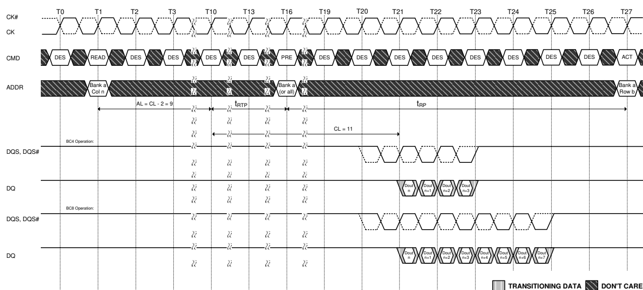
Figure 118. READ to PRECHARGE with Additive Latency and 1t CK Preamble
