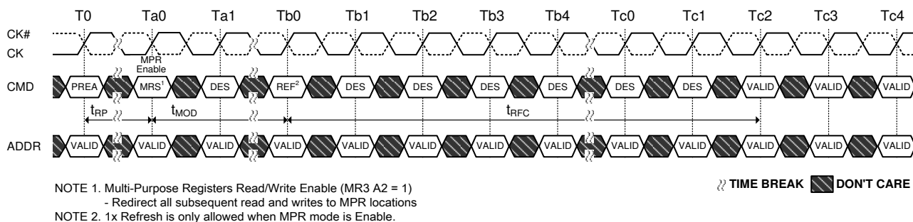
Figure 70. Refresh Command Timing
