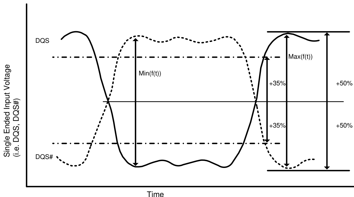
Figure 209. Definition of differential DQS Peak Voltage and rage of exempt non-monotonic signaling
