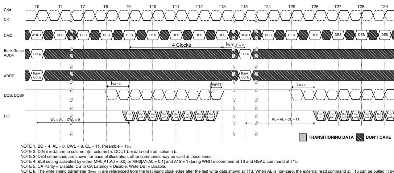
Figure 141. WRITE (BL8) to READ (BL8) with 1t CK Preamble in Different Bank Group
