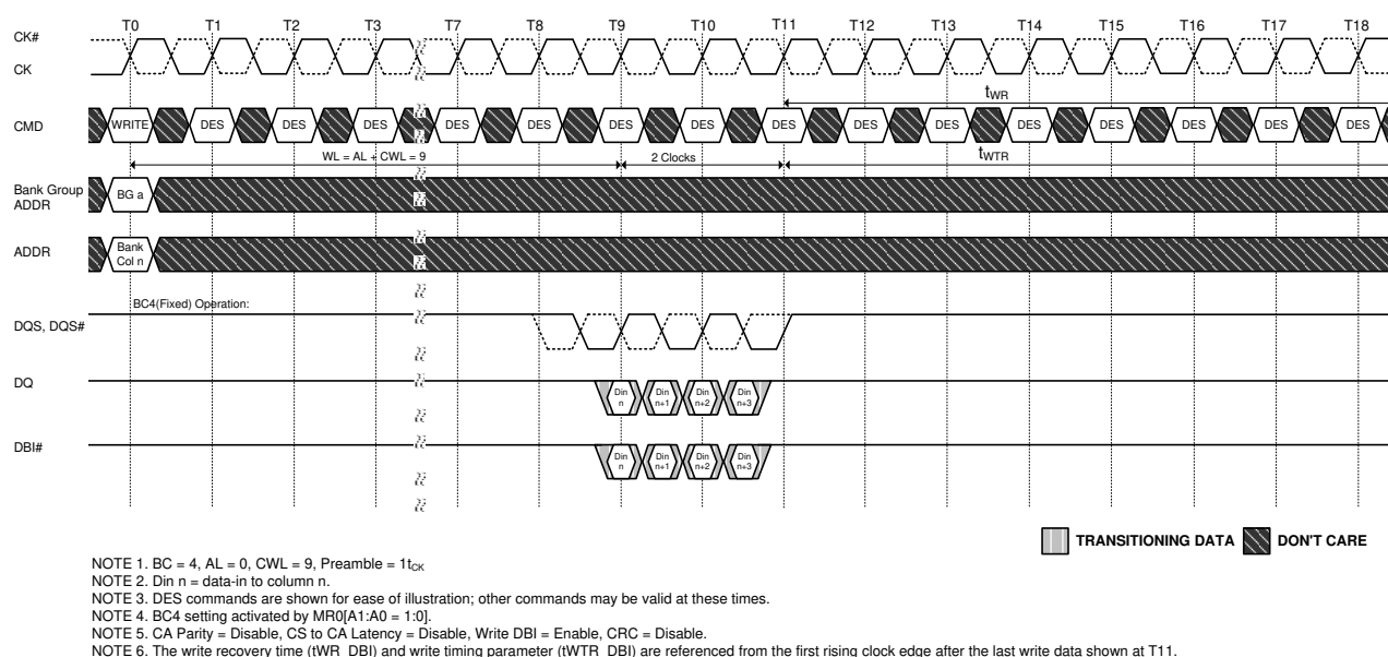
Figure 154. WRITE (BC4) Fixed with 1t_{CK} Preamble and DBI
