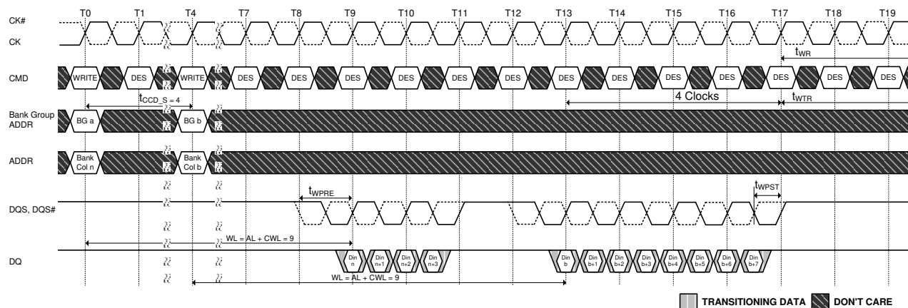
Figure 147. WRITE (BL8) to WRITE (BC4) OTF with 1t CK Preamble in Different Bank Group
