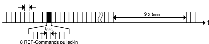
Figure 43. Pulling-in Refresh Commands (Example of 1X Refresh mode)
