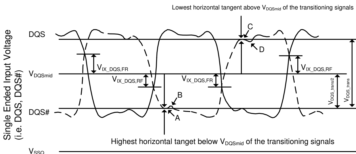
Figure 210. Vix Definition (DQS)
