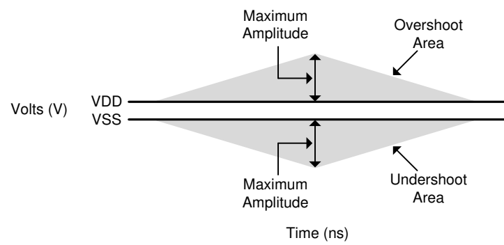
Figure 51. AC Overshoot and Undershoot Definition for Address and Control Pins
