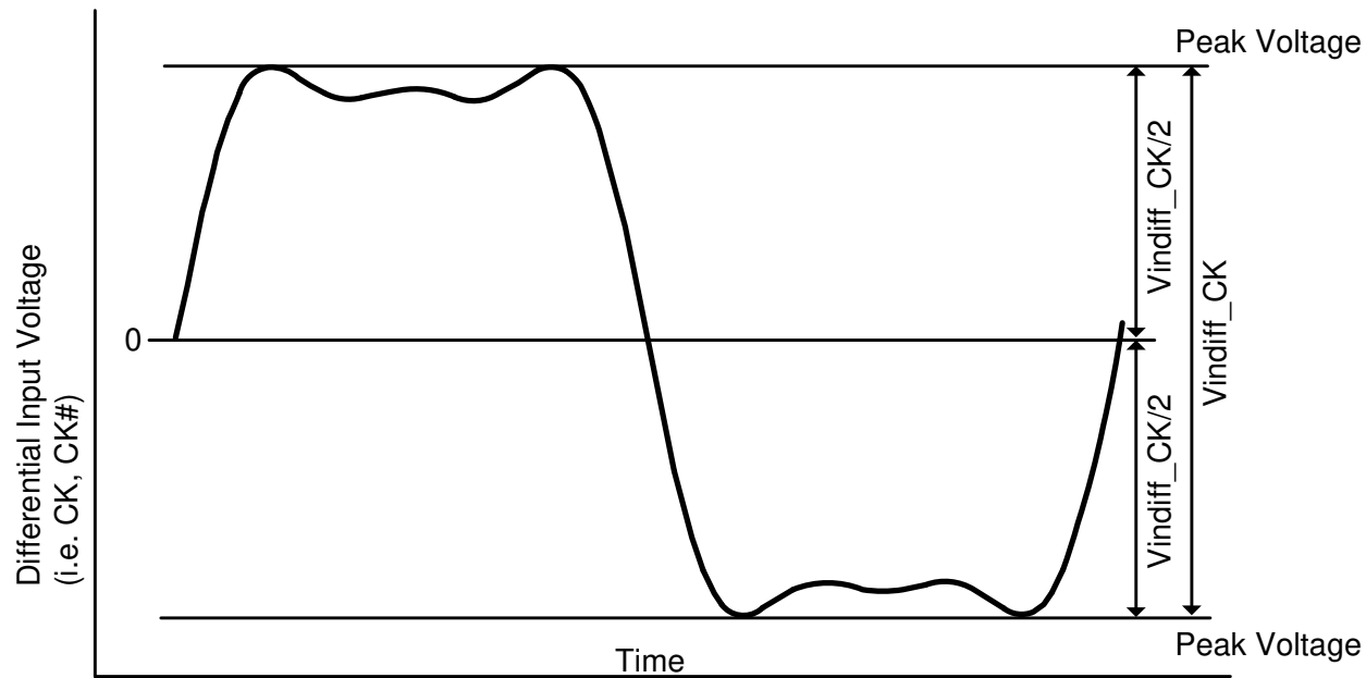
Figure 52. CK Differential Input Voltage
