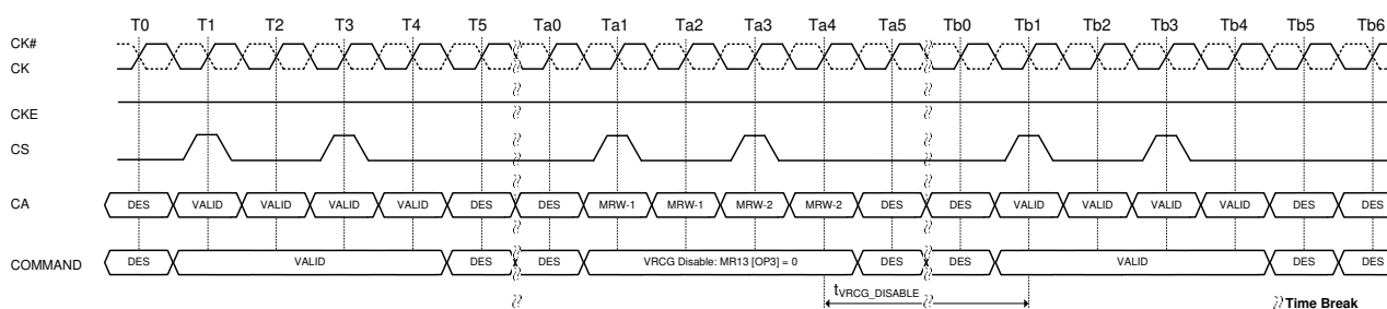
Figure 32. VRCG Disable timing
