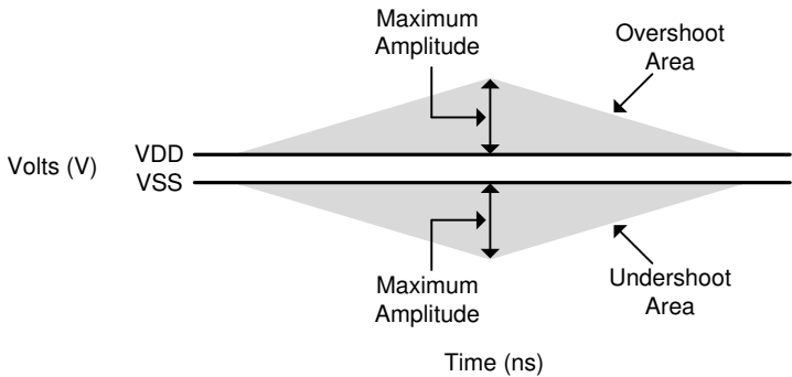
Figure 62. Overshoot and Undershoot Definition
