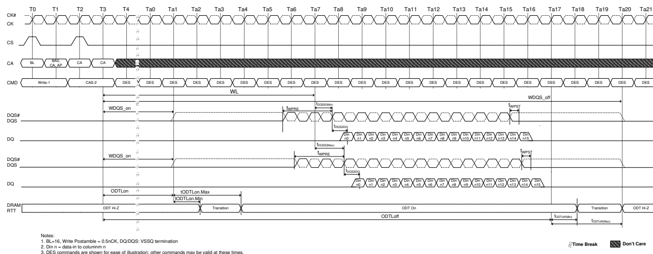
Figure 26. Asynchronous ODTon/ODToff Timing
