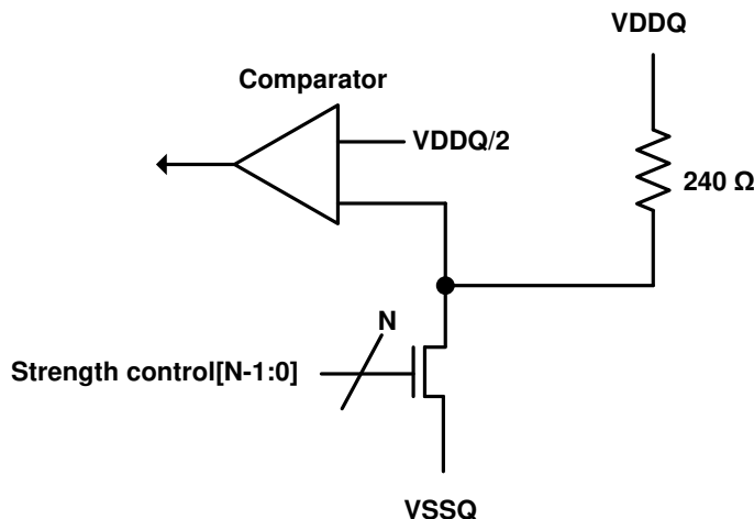
Figure 65. Pull-down calibration
