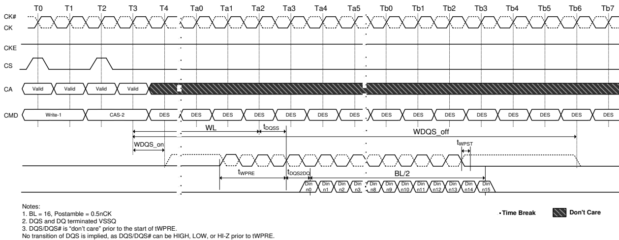
Figure 13. DQS Write Preamble and Postamble: 0.5nCK Postamble
