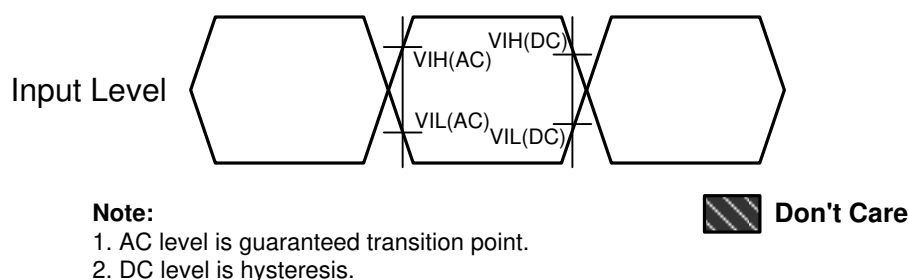
Figure 49. Input AC timing definition for CKE
