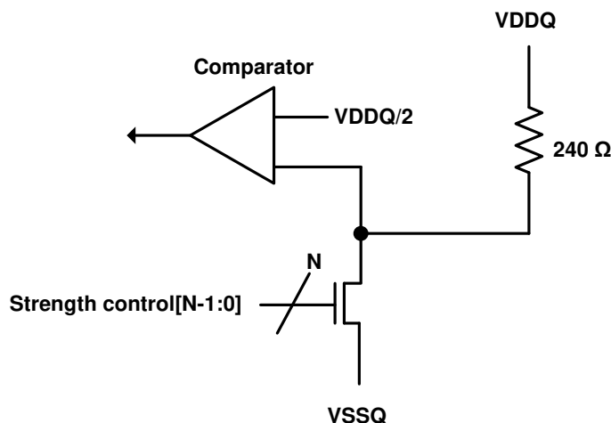
Figure 65. Pull-down calibration
