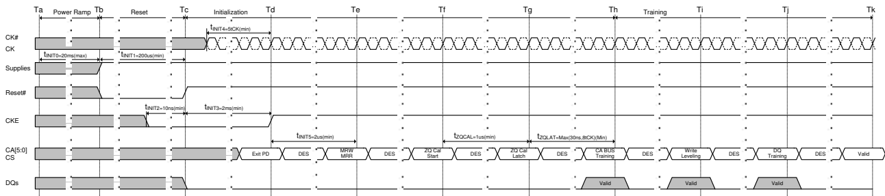
Figure 5. Power Ramp and Initialization Sequence
