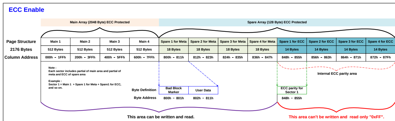
Figure 1-3. Architecture and Address of Page Size 2048+128 bytes
