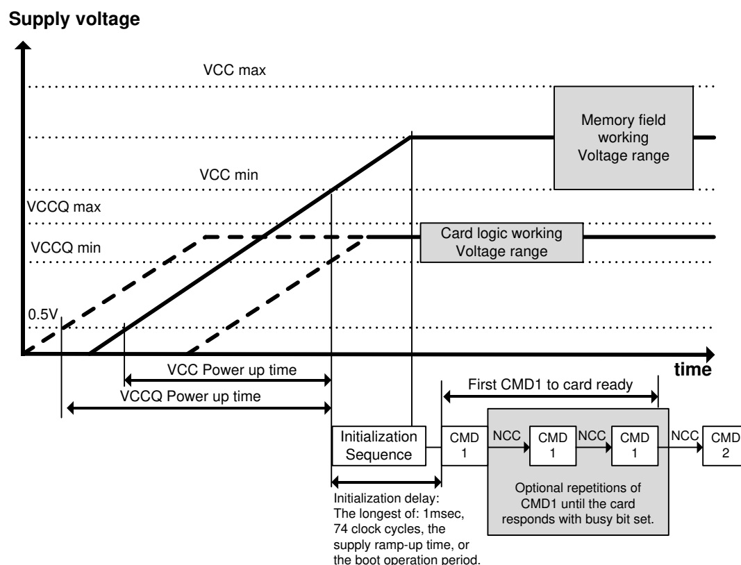
Figure 7-2. Power-up Diagram
