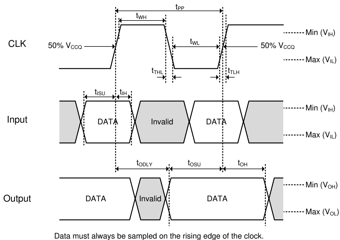
Figure 7-8. Timing Diagram
