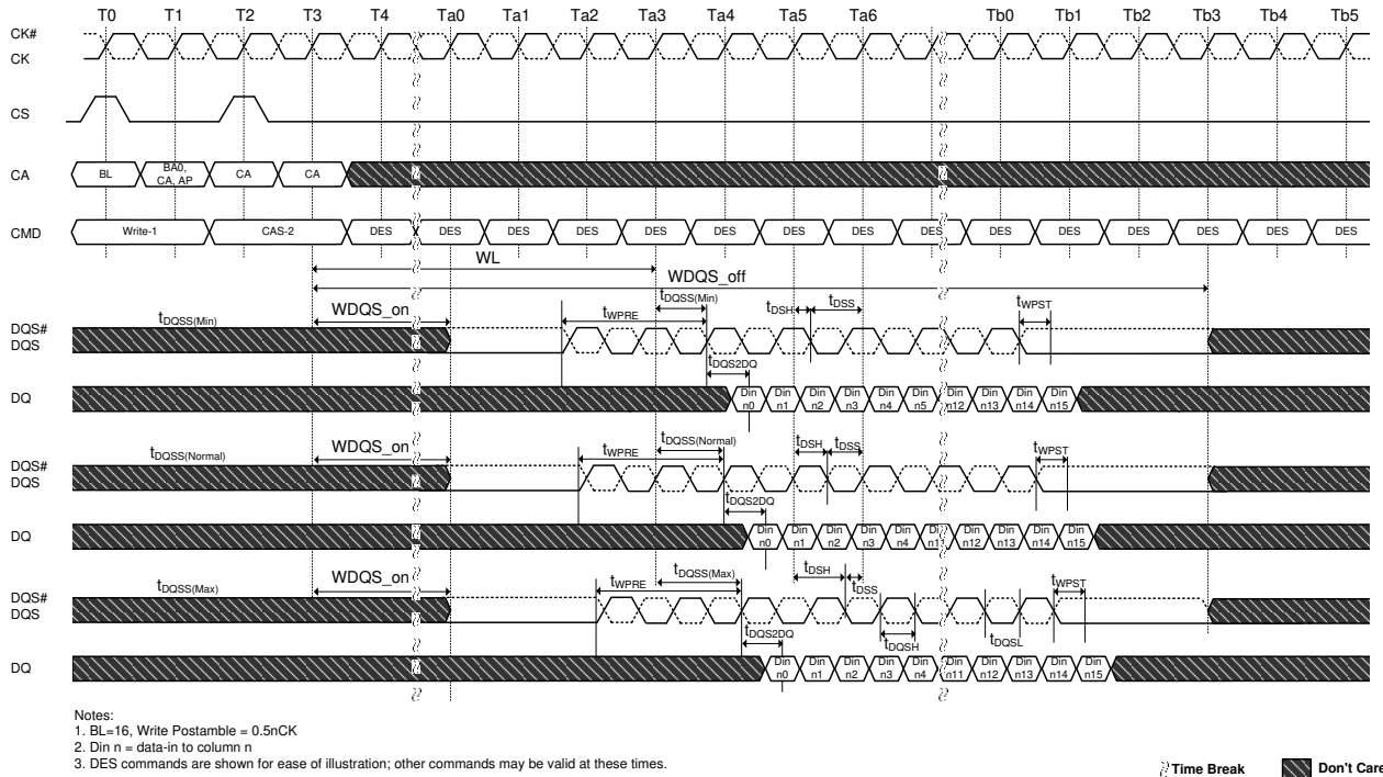
Figure 17. Write Timing
