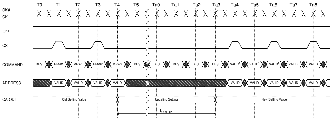
Figure 27. ODT for Command/Address setting update timing in 4 Clock Cycle Command
