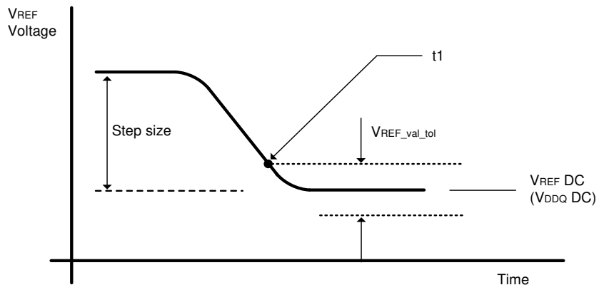
Figure 44. VREF step single step size decrement case
