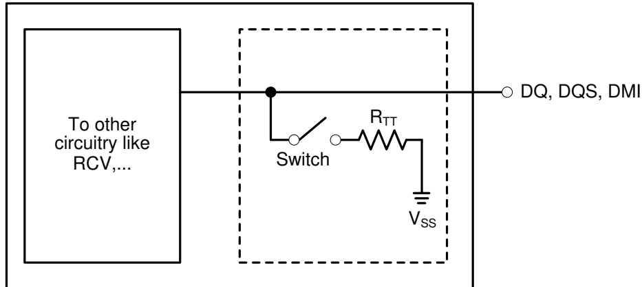
Figure 22. Functional Representation of ODT
