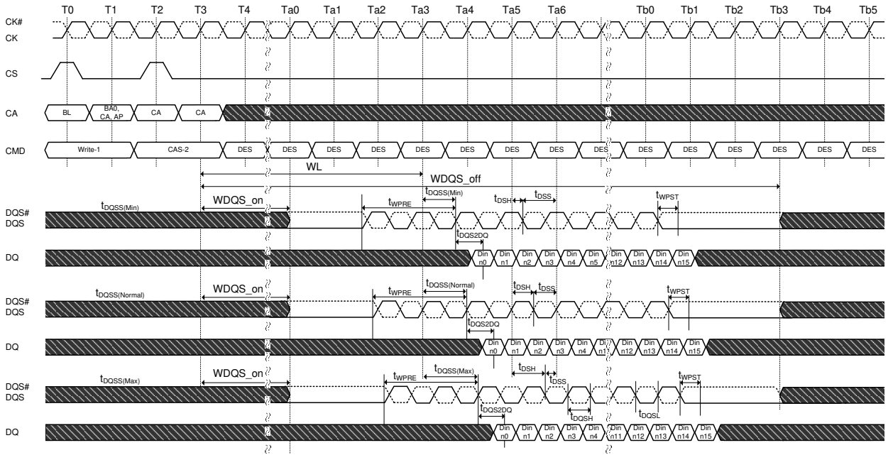
Figure 17. Write Timing
