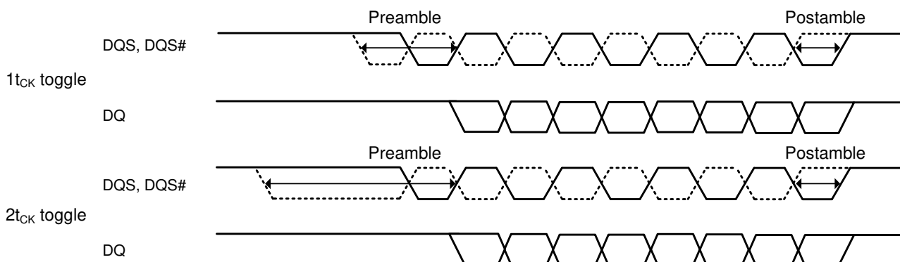
Figure 90. Read Postamble
