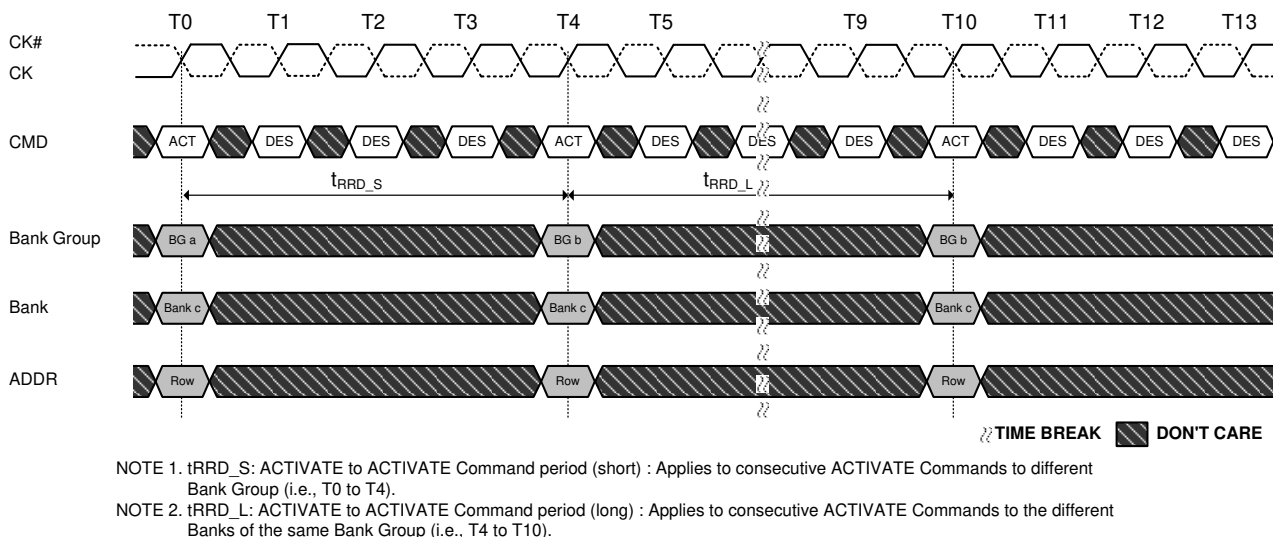
Figure 80. t_{RRD} Timing
