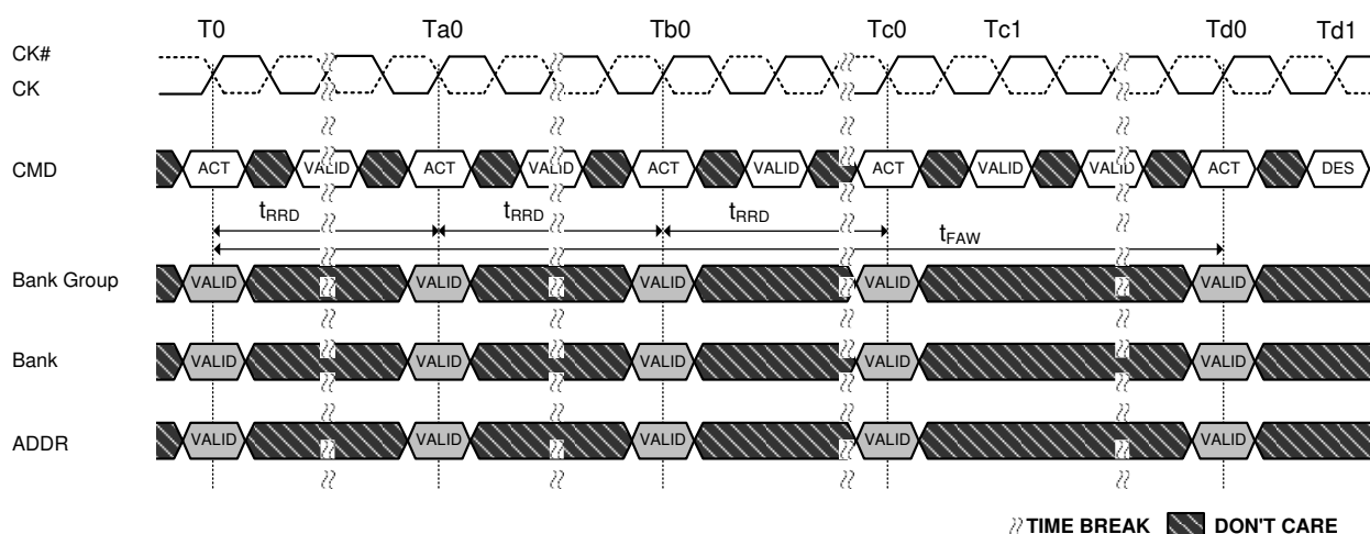
Figure 81. t_FAW Timing
