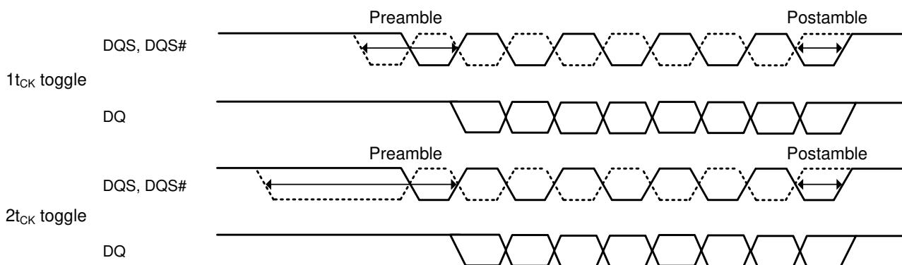
Figure 90. Read Postamble
