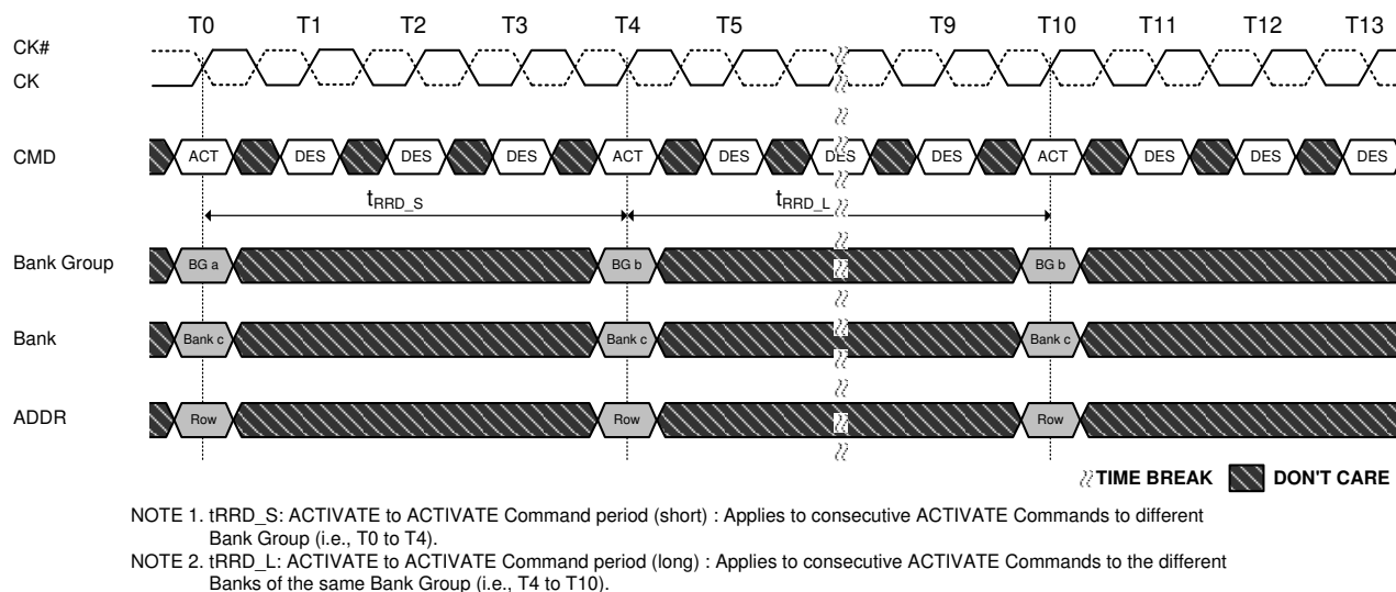
Figure 80. t_{RRD} Timing
