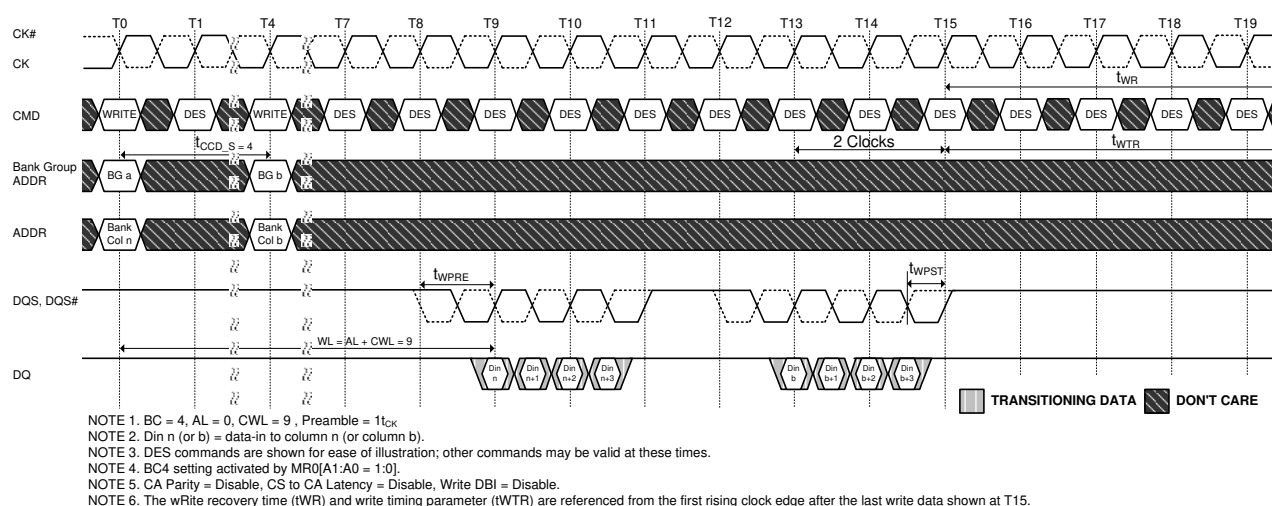
Figure 145. Write (BC4) Fixed to Write (BC4) Fixed with 1t_{CK} Preamble in Different Bank Group
