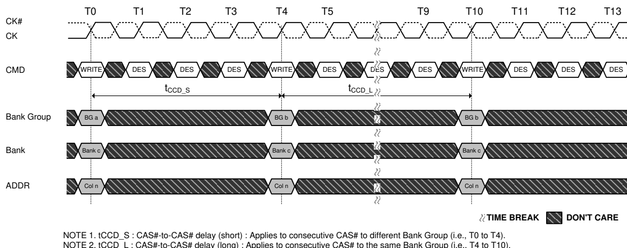
Figure 78. t_{ccd} Timing (Write to Write Example)
