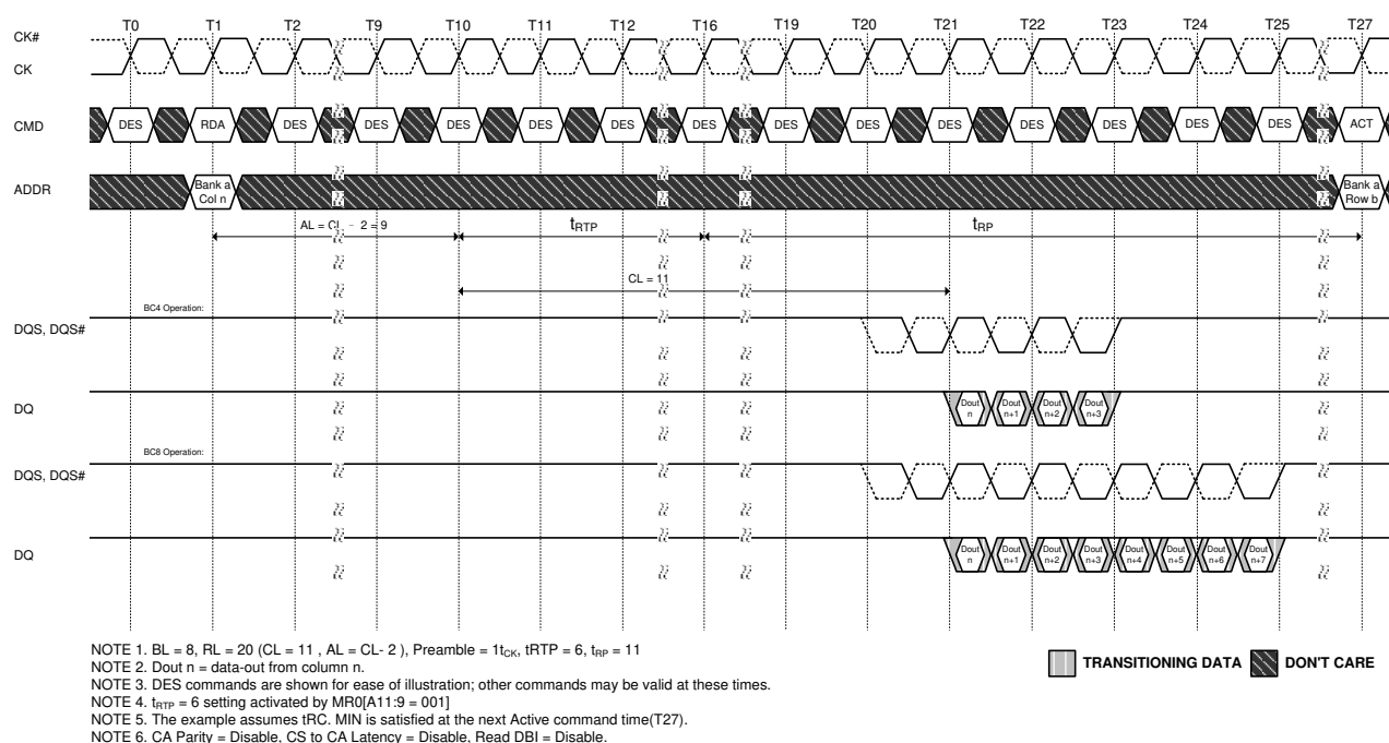
Figure 125. Read with Auto Precharge, Additive Latency and 1tck Preamble
