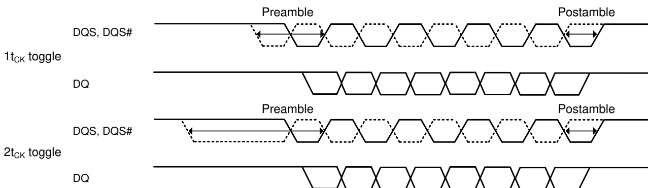
Figure 91. Write Postamble
