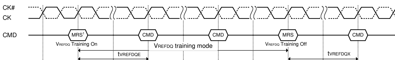
Figure 53. VREFDQ training mode entry and exit timing diagram
