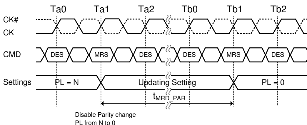
Figure 67. Parity entry timing example - t_{MOD\_PAR}
