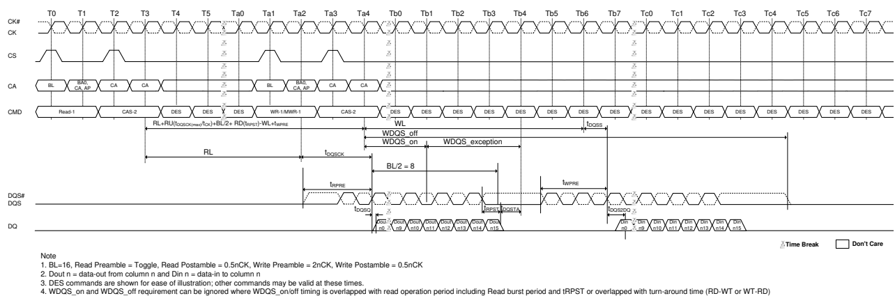
Figure 19. Burst Write Operation
