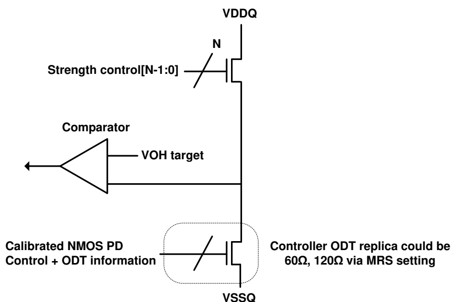
Figure 66. Pull-up calibration
