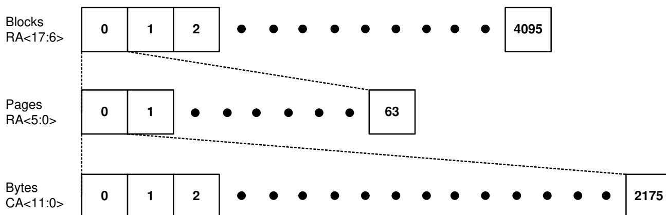
Figure 1-2. Memory Mapping Diagram for EM73E044VCE-H
