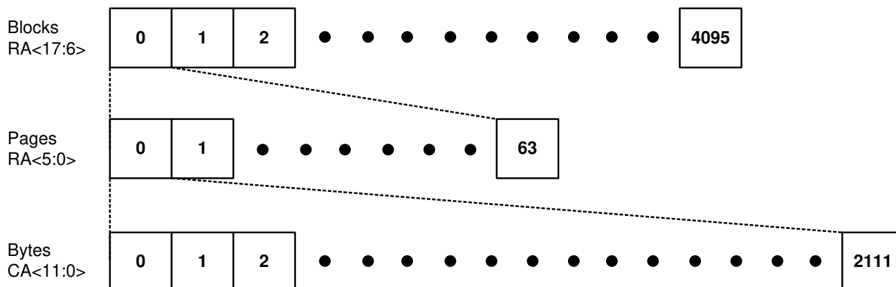
Figure 1-3. Memory Mapping Diagram for EM73E044VCG-H
