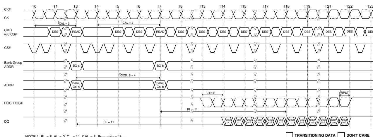
Figure 127. Consecutive READ (BL8) with CAL(3) and 1t CK Preamble in Different Bank Group
