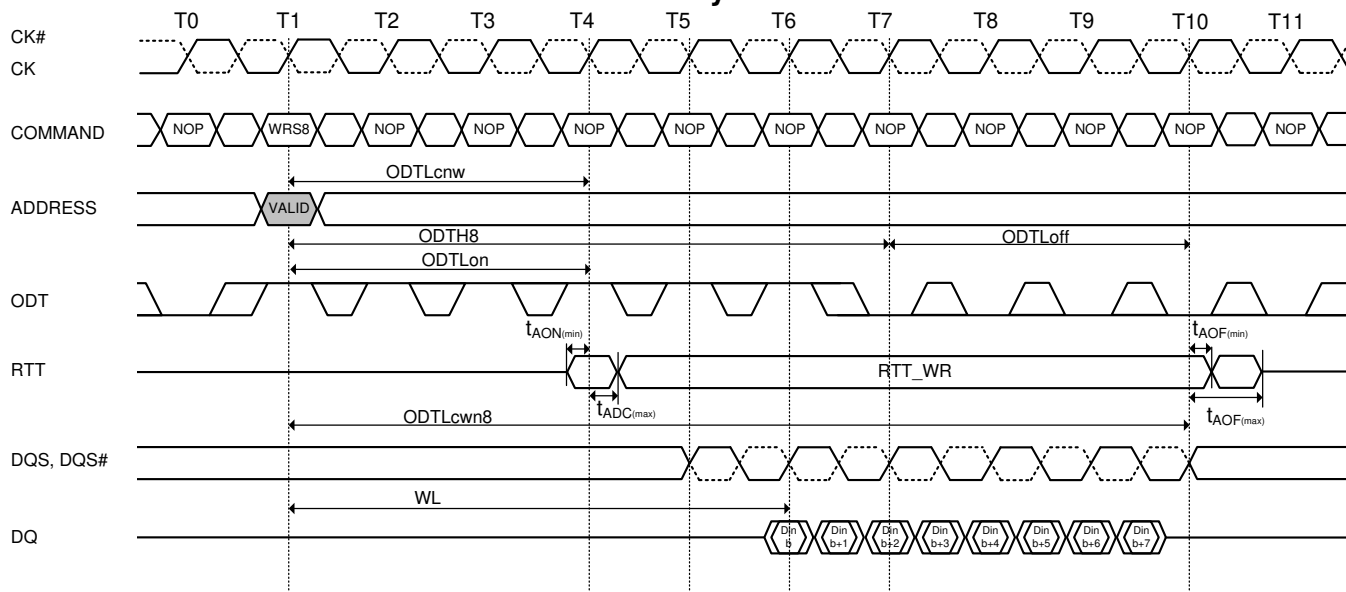
Figure 93. Dynamic ODT: Behavior with ODT pin being asserted together with write command for a duration of 6 clock cycles
