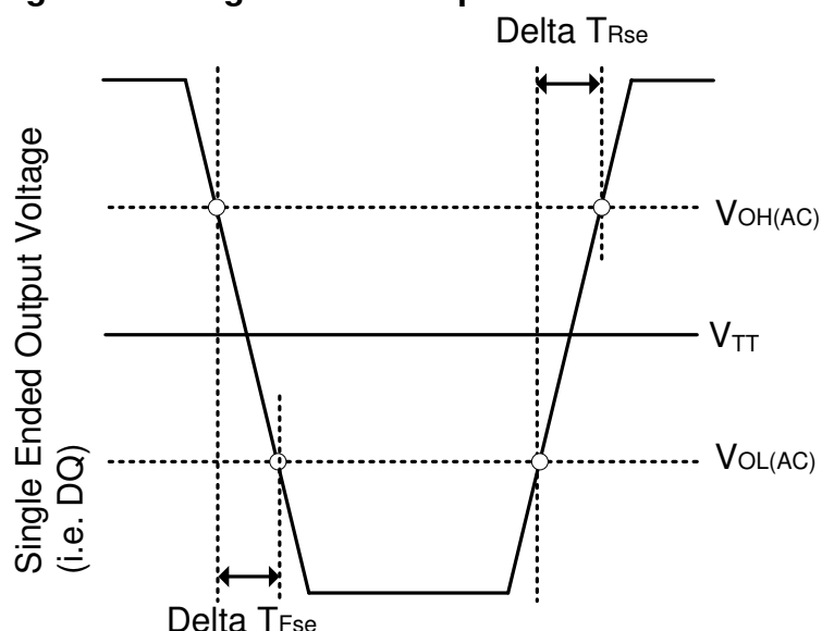
Figure 37. Single-ended Output Slew Rate Definition
