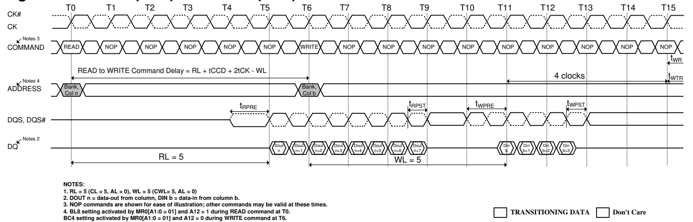
Figure 62. READ (BL8) to WRITE (BL4) OTF
