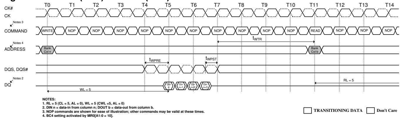
Figure 75. WRITE(BC4) to READ(BC4)
