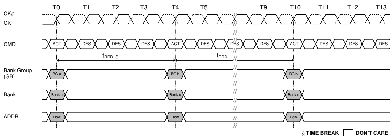
Figure 76. t_{RRD} Timing
