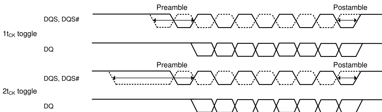
Figure 90. Read Postamble
