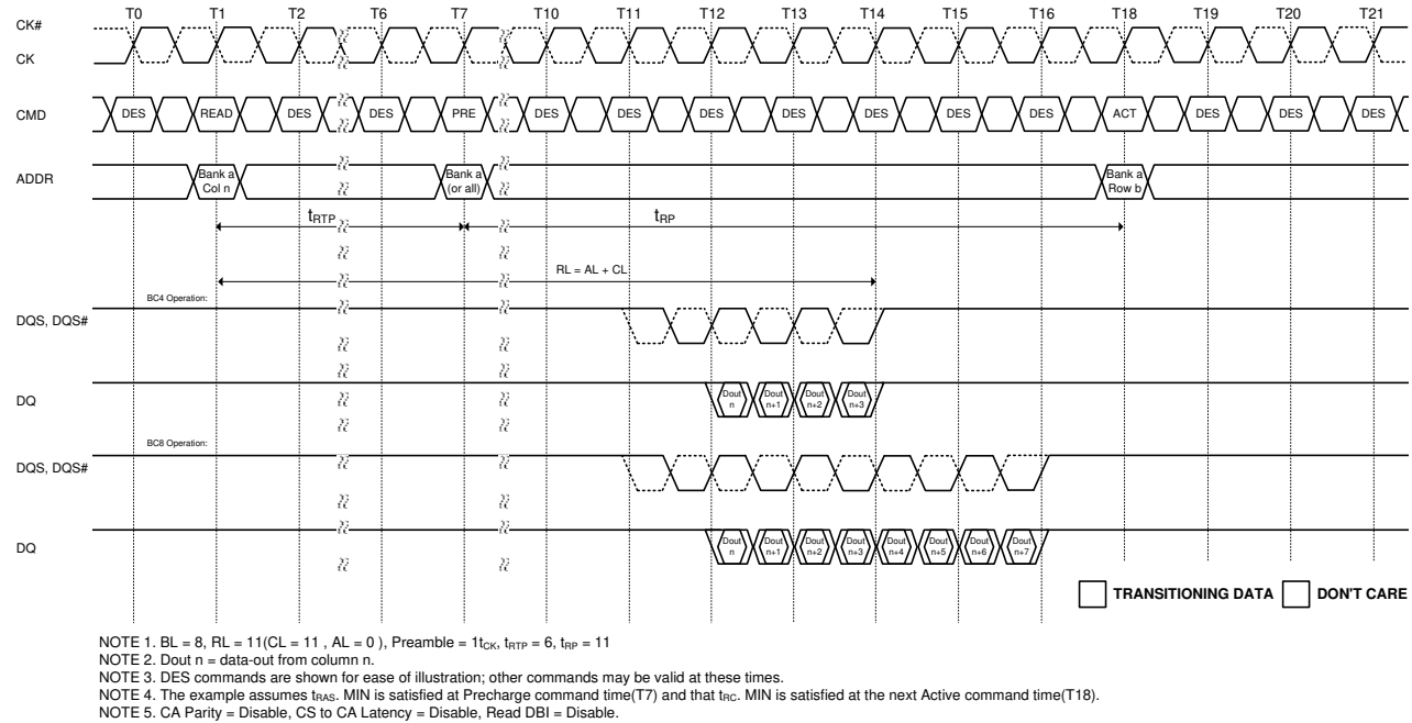
Figure 21. Read to Precharge with 1t_{CK} Preamble
