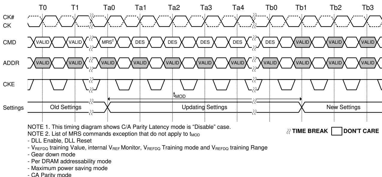
Figure 7. t_{MOD} timing
