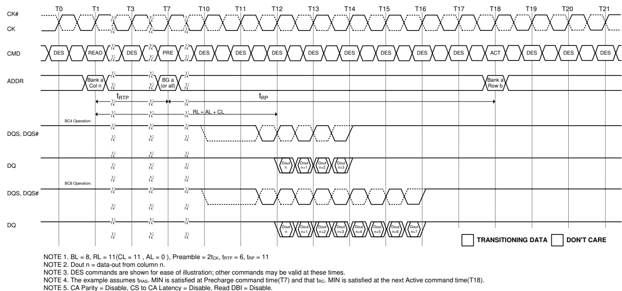
Figure 22. Read to Precharge with 2t_{CK} Preamble
