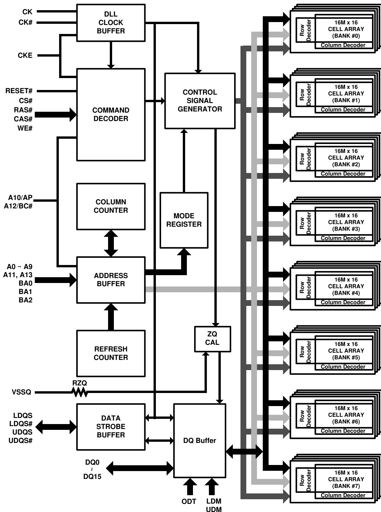
Figure 2. Block Diagram
