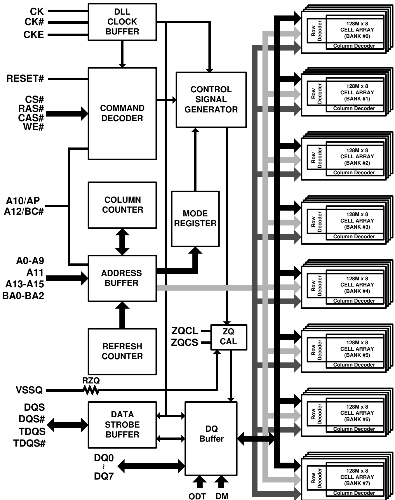
Figure 2. Block Diagram
