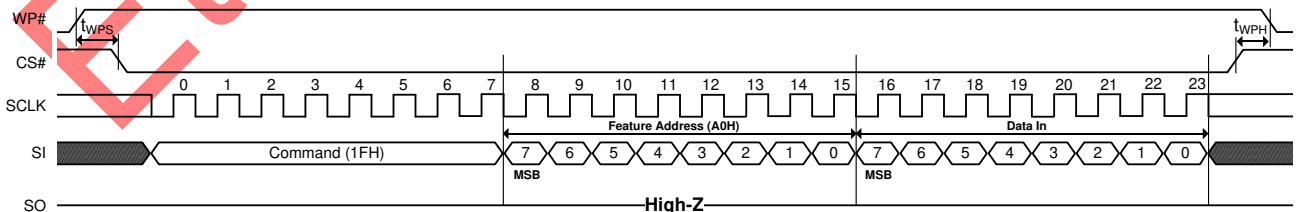
Figure 16-4. WP# Timing
