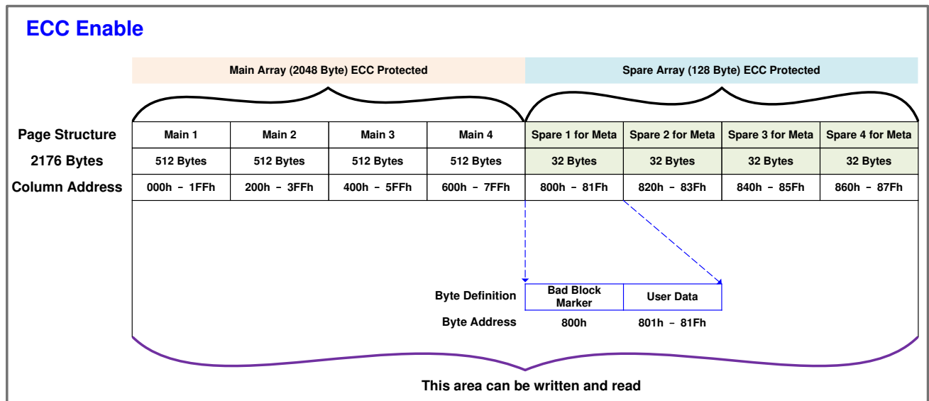
Figure 1-5. Architecture and Address of Page Size 2048+128 bytes
