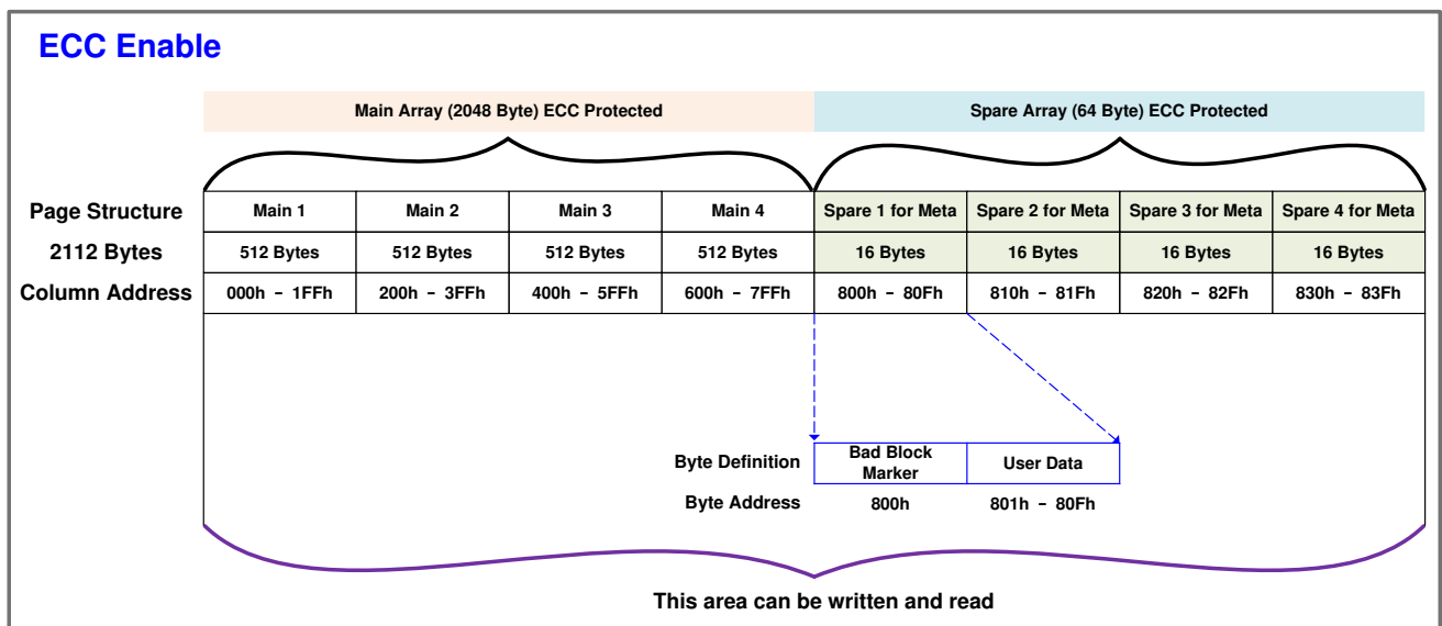
Figure 1-5. Architecture and Address of Page Size 2048+64 bytes
