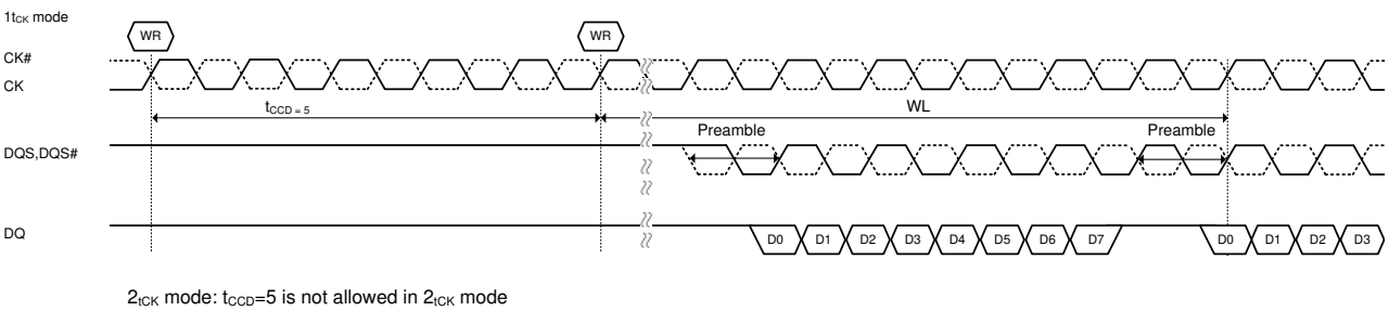
Figure 82. t_{CCD}=5 (AL=PL=0)
