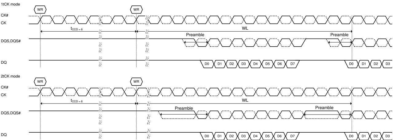
Figure 83. t_{CCD}=6 (AL=PL=0)
