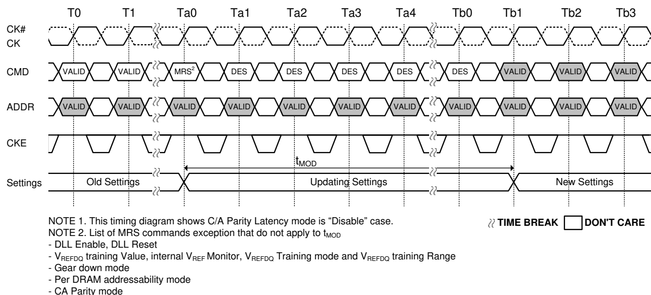
Figure 7. t_{MOD} timing
