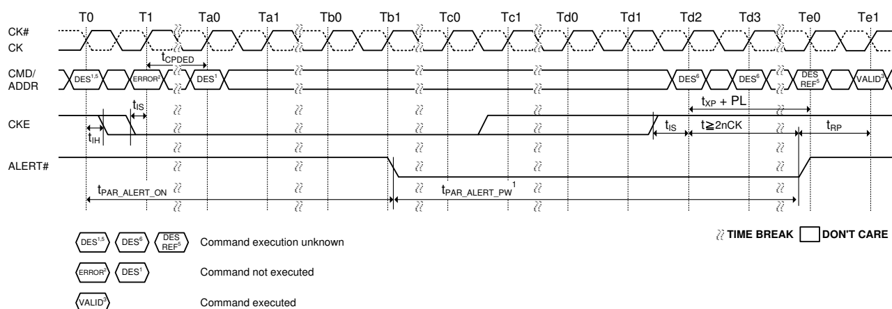
Figure 59. CA Parity Error Checking - PDE/PDX
