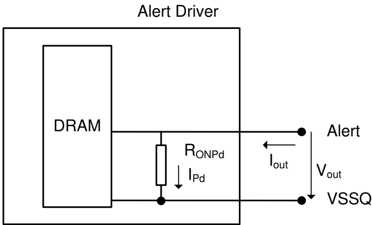
Figure 199. ALERT# output Drive Characteristic
