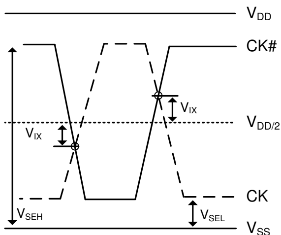
Figure 204. Vix Definition (CK)
