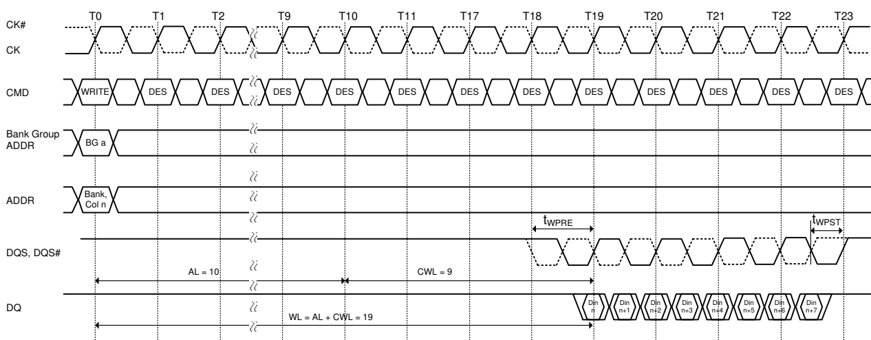
Figure 137. WRITE Burst Operation WL = 9 (AL = 0, CWL = 9, BL8)
