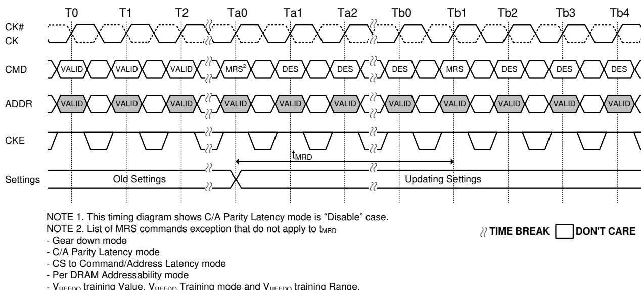
Figure 6. t_{MRD} timing
