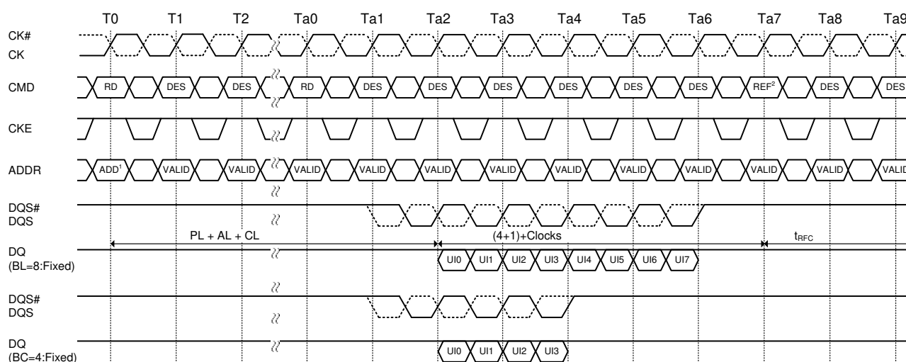
Figure 75. Refresh Command Timing
