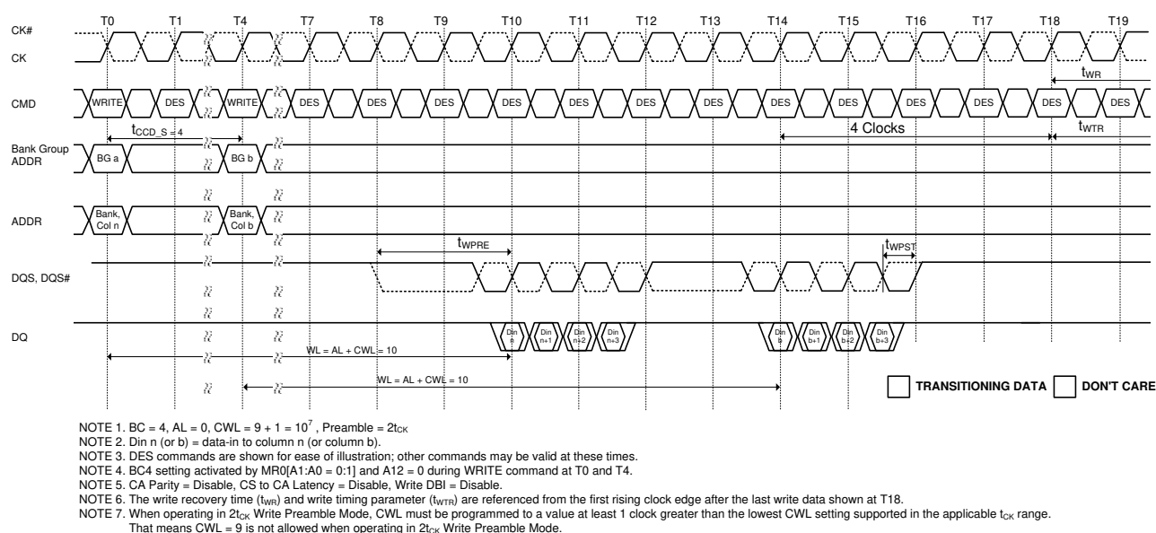
Figure 144. WRITE (BC4) OTF to WRITE (BC4) OTF with 2tCK Preamble in Different Bank Group
