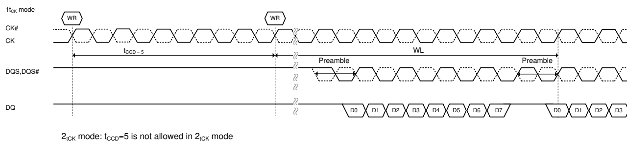
Figure 86. tCCD=5 (AL=PL=0)
