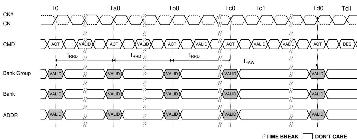
Figure 81. tFAW Timing
