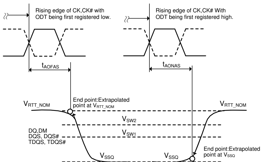
Figure 184. Definition of t_{\text{AOFAS}} and t_{\text{AONAS}}
