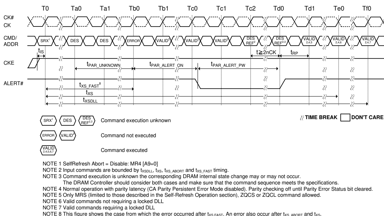
Figure 65. CA Parity Error Checking - SRX
