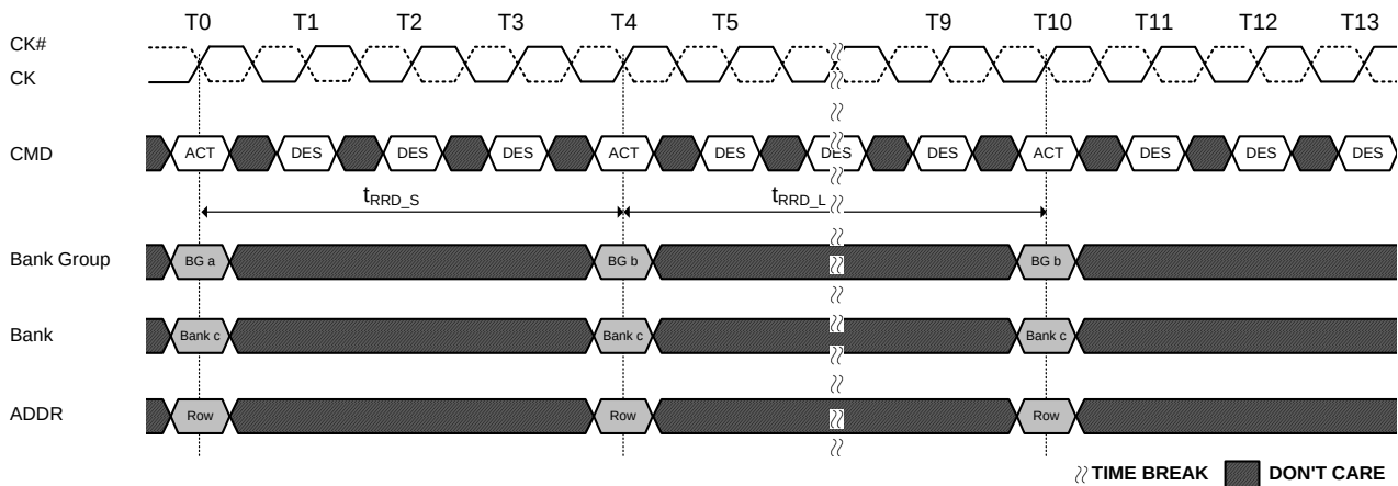
Figure 80. tRRD Timing
