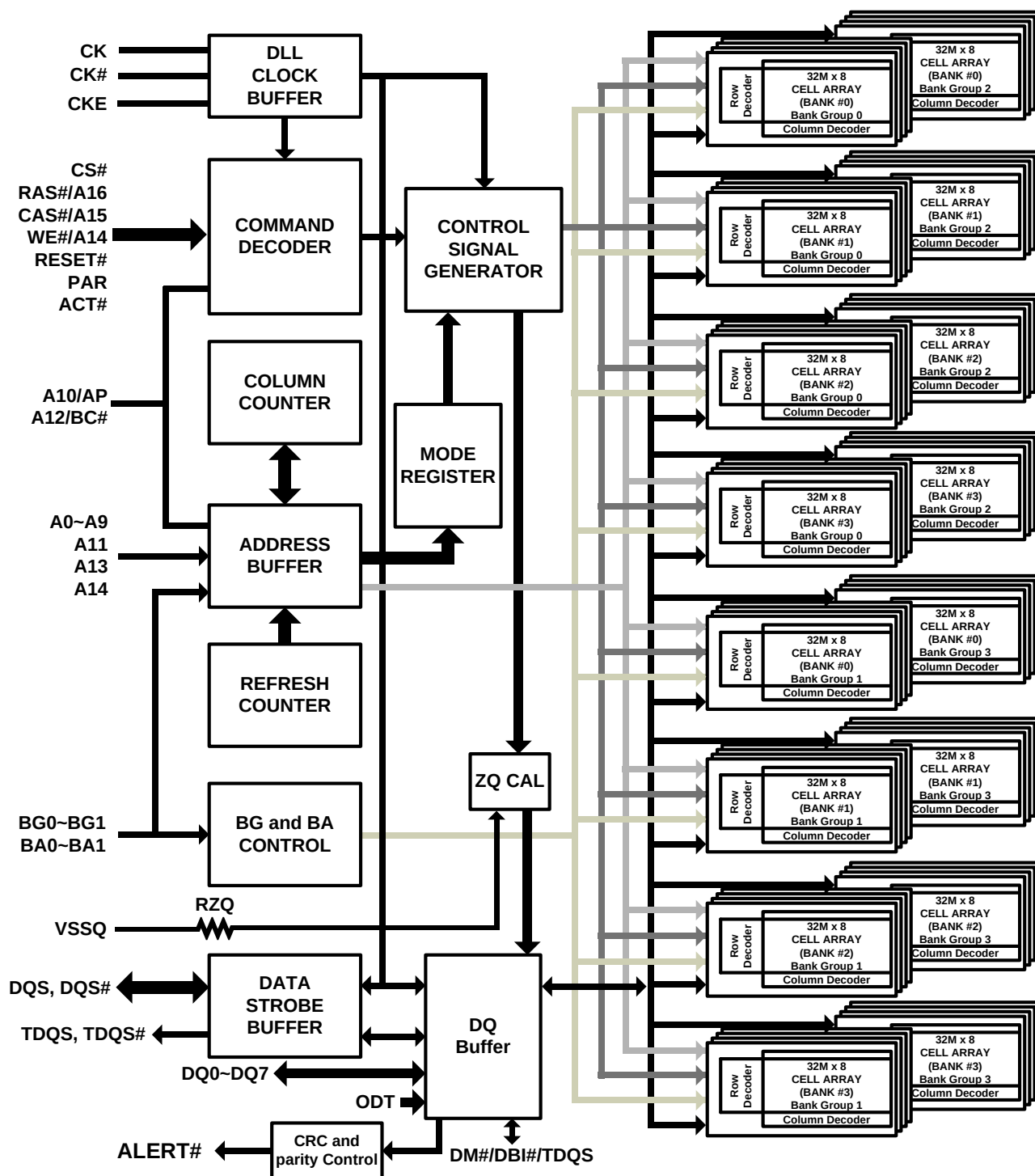
Figure 2. Block Diagram
