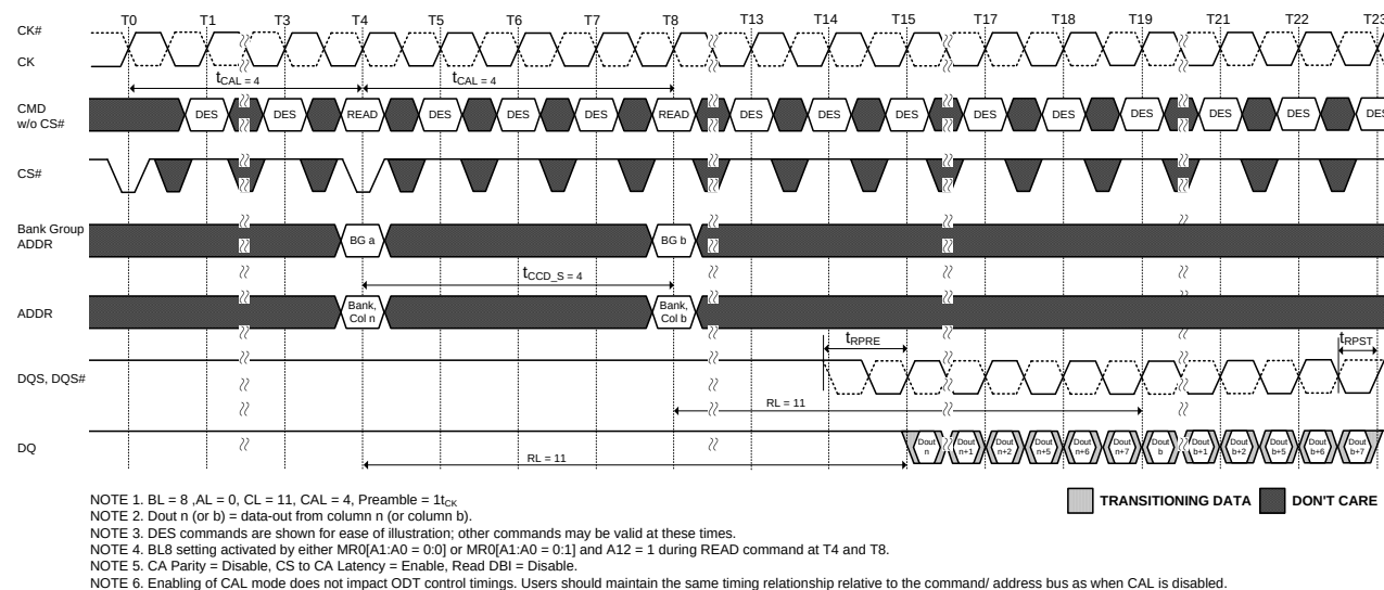
Figure 132. Consecutive READ (BL8) with CAL(4) and 1tCK Preamble in Different Bank Group
