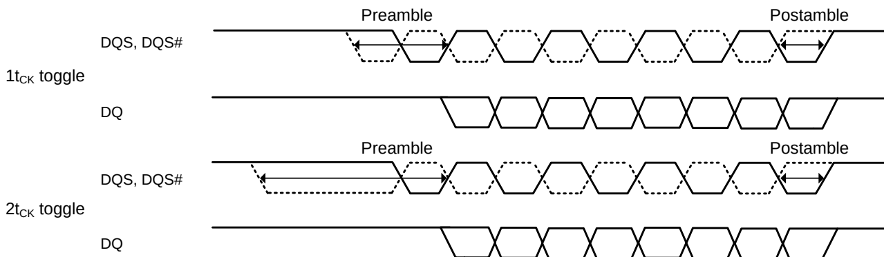
Figure 90. READ Postamble
