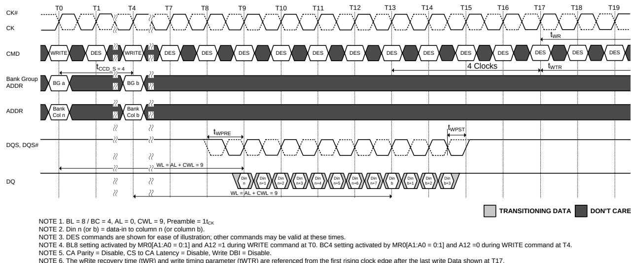
Figure 152. WRITE (BL8) to WRITE (BC4) OTF with 1tCK Preamble in Different Bank Group
