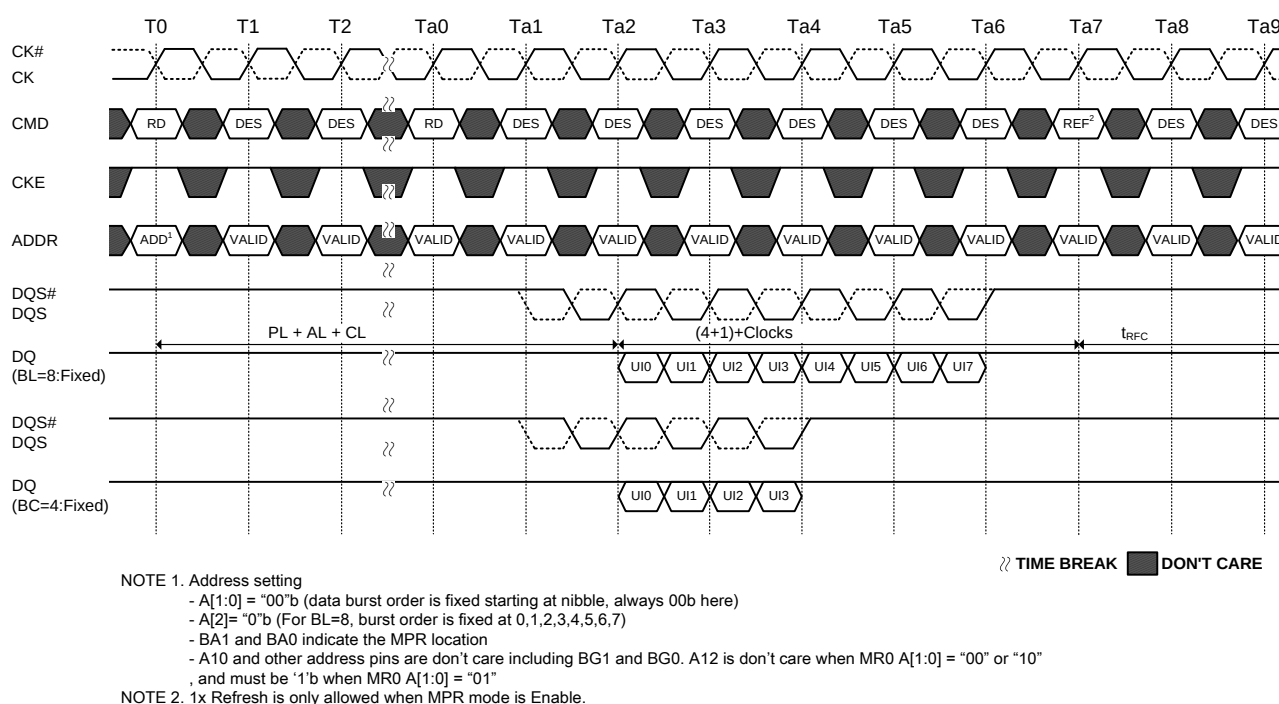
Figure 76. Read to Refresh Command Timing
