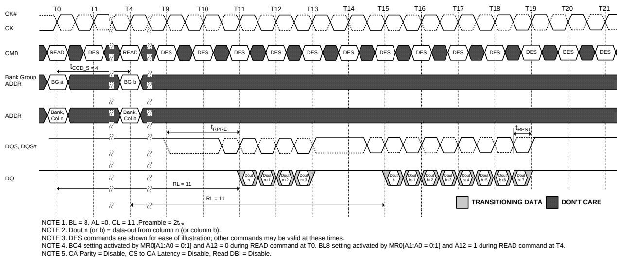
Figure 116. READ (BC4) to READ (BL8) OTF with 2tCK Preamble in Different Bank Group
