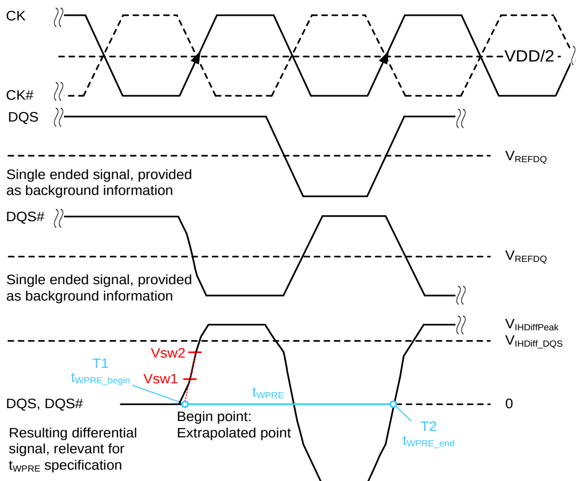
Figure 135. Method for calculating t_{WPRE} transitions and endpoints
