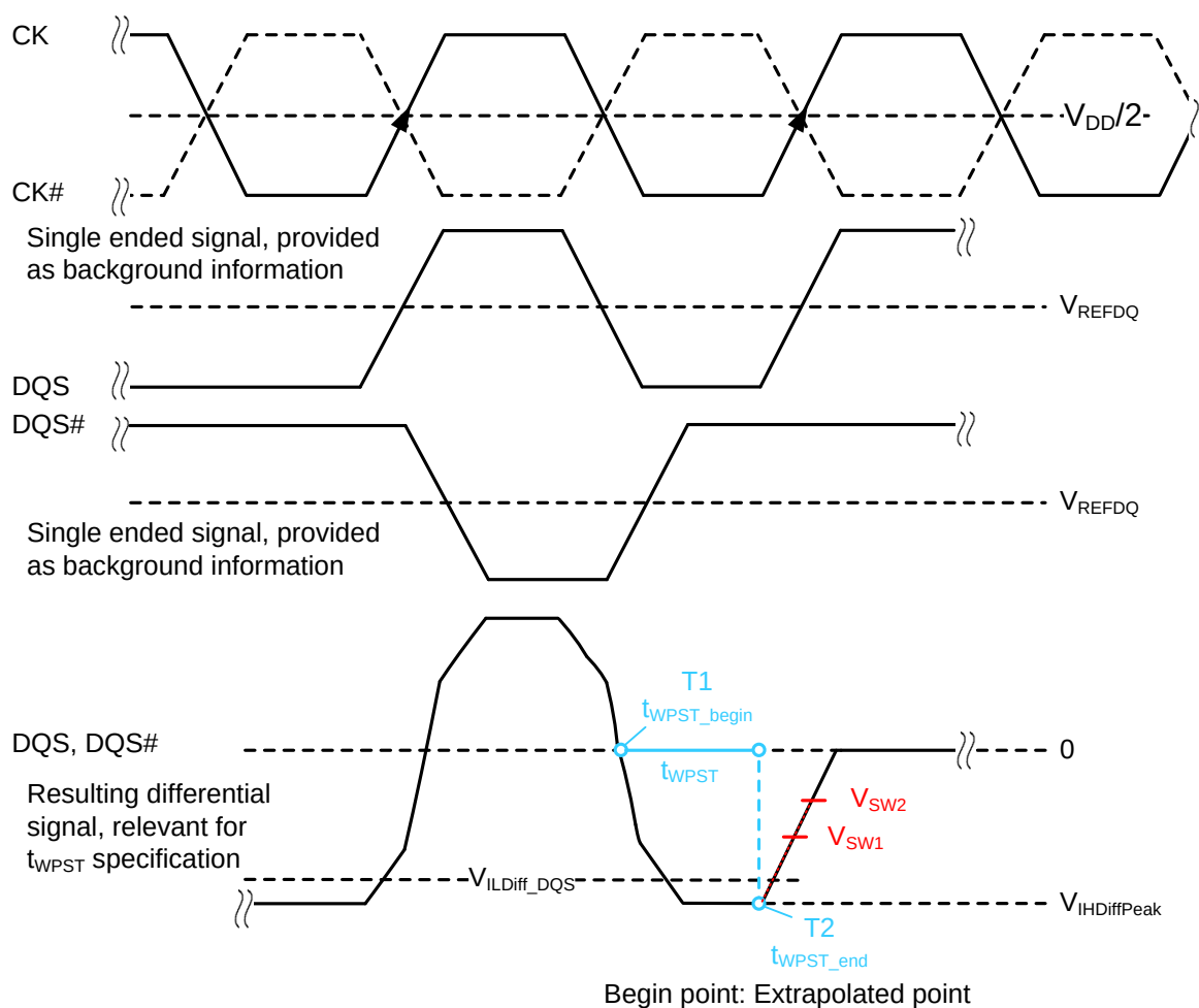
Figure 136. Method for calculating t_{WPST} transitions and endpoints
