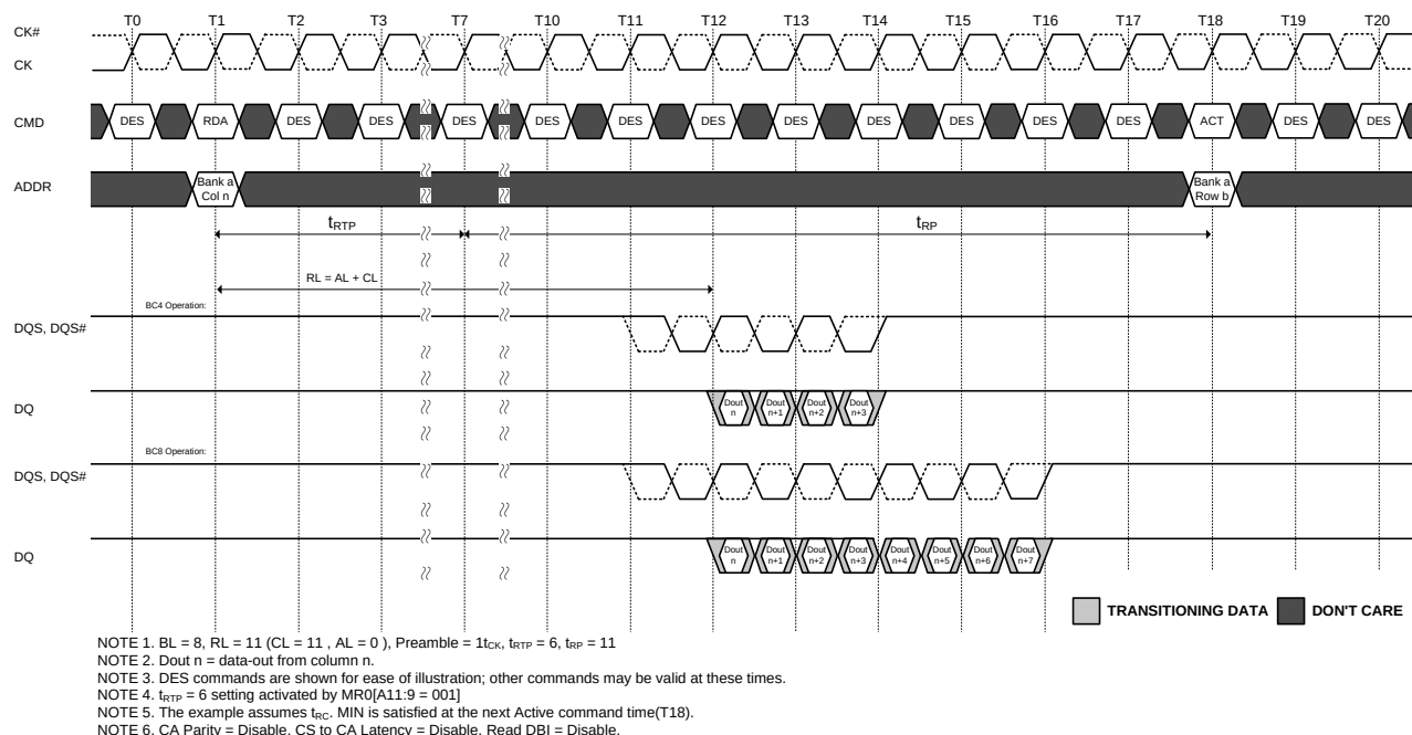
Figure 124. READ with Auto Precharge and 1tCK Preamble
