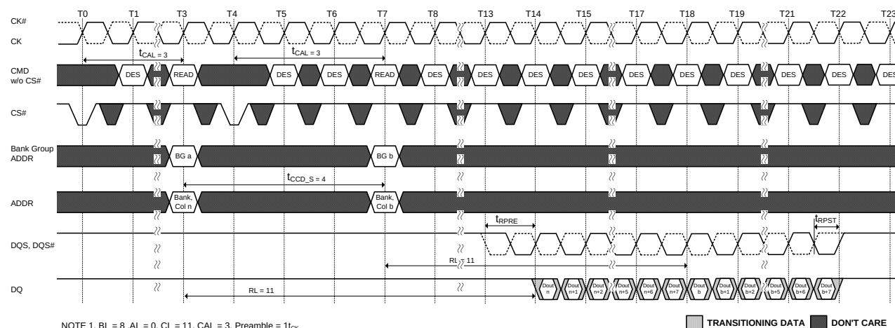
Figure 131. Consecutive READ (BL8) with CAL(3) and 1tCK Preamble in Different Bank Group
