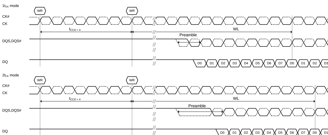
Figure 85. t_{CCD}=4 (AL=PL=0)
