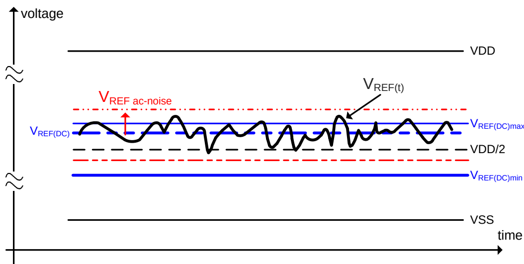
Figure 185. Illustration of V_{REF}(DC) tolerance and V_{REF} AC-noise limits
