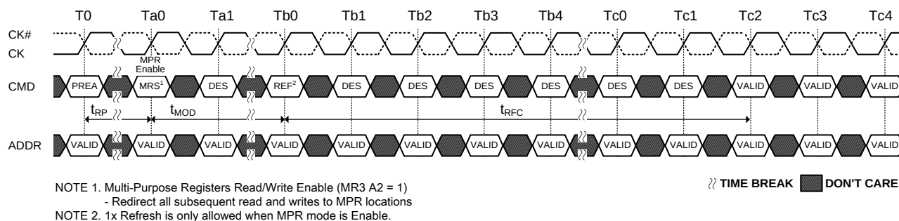
Figure 75. Refresh Command Timing
