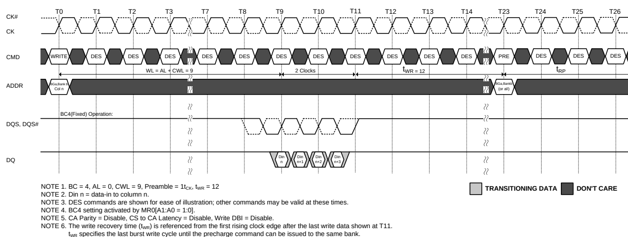
Figure 155. WRITE (BC4) Fixed to PRECHARGE Operation with 1tCK Preamble
