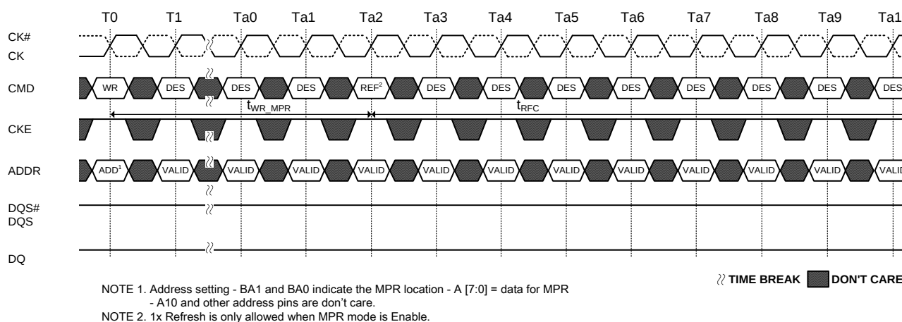
Figure 77. Write to Refresh Command Timing
