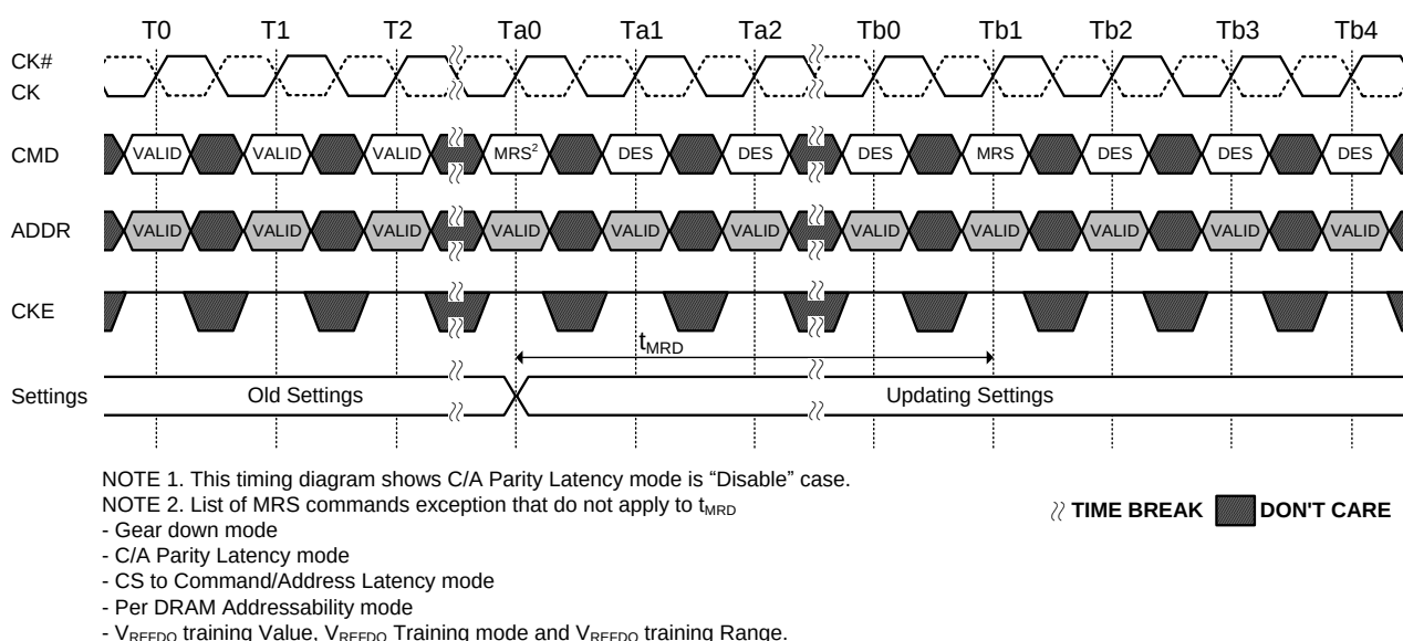
Figure 6. t_{MRD} timing
