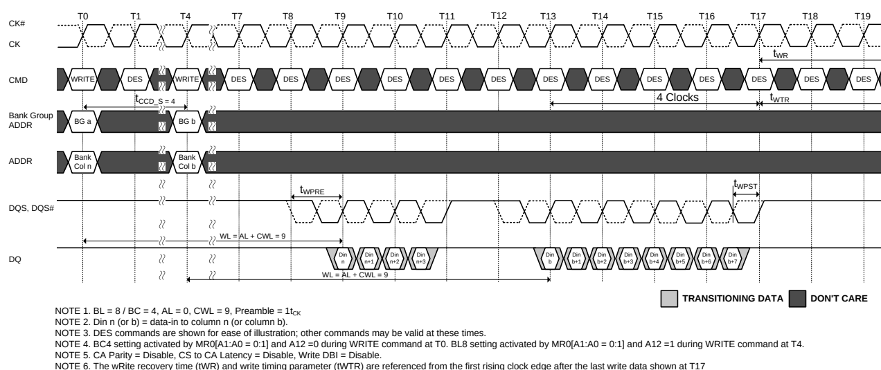
Figure 153. WRITE (BC4)OTF to WRITE (BL8) with 1tCK Preamble in Different Bank Group
