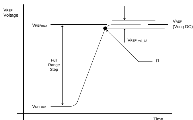
Figure 56. VREF full step from VREFmin to VREFmax case
