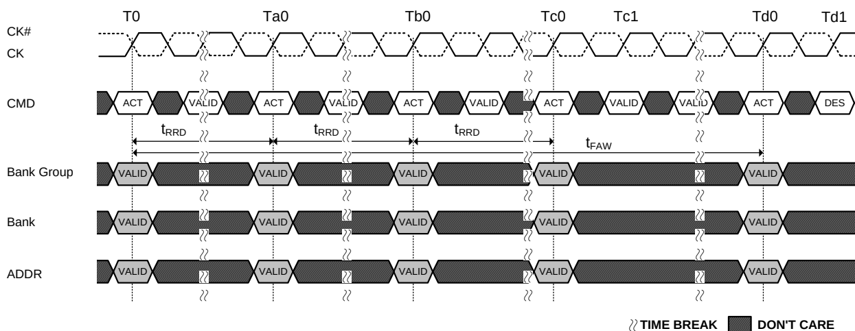
Figure 81. tFAW Timing
