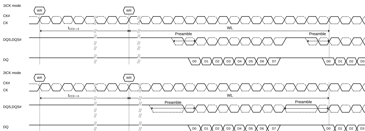
Figure 87. t CCD =6 (AL=PL=0)
