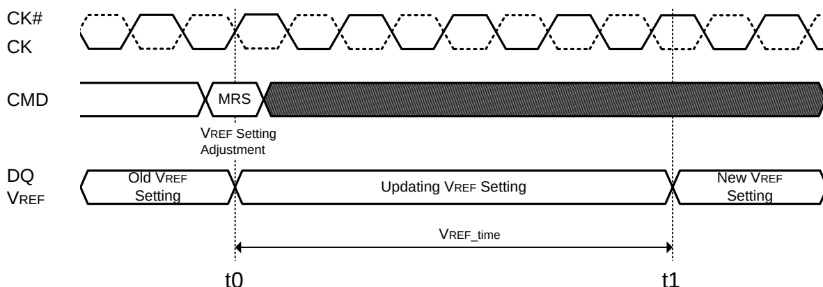
Figure 52. V_{REF\_time} timing diagram
