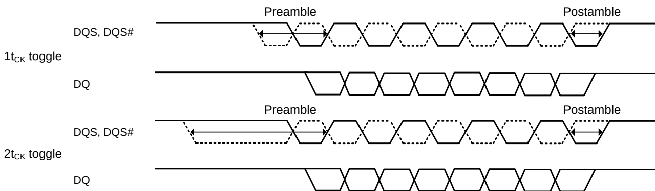
Figure 91. WRITE Postamble
