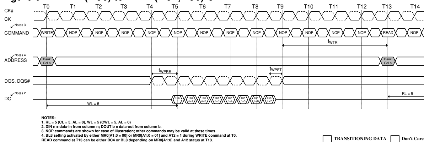
Figure 52. WRITE(BC8) to READ(BC4,BC8) OTF
