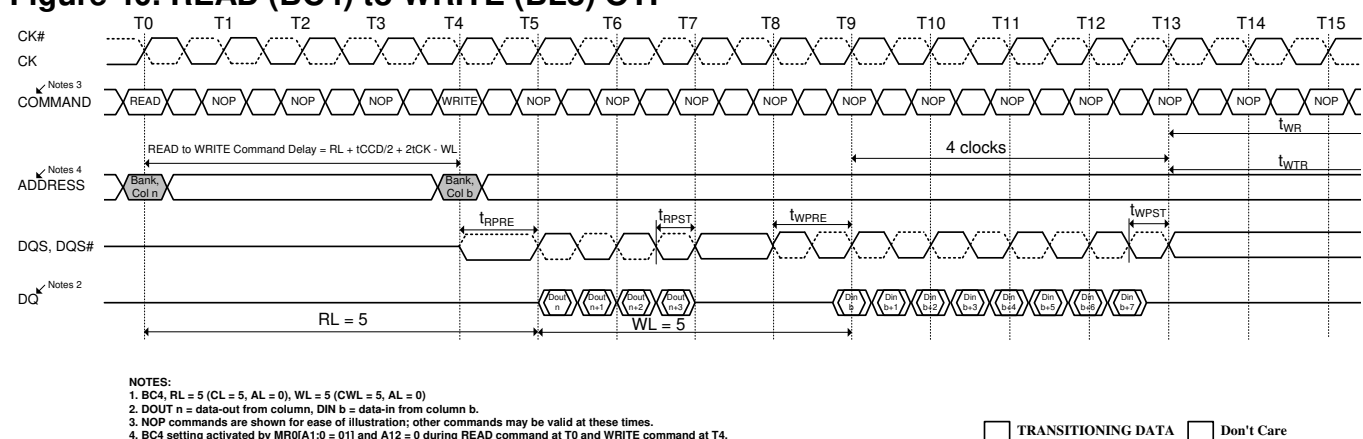
Figure 40. READ (BC4) to WRITE (BL8) OTF
