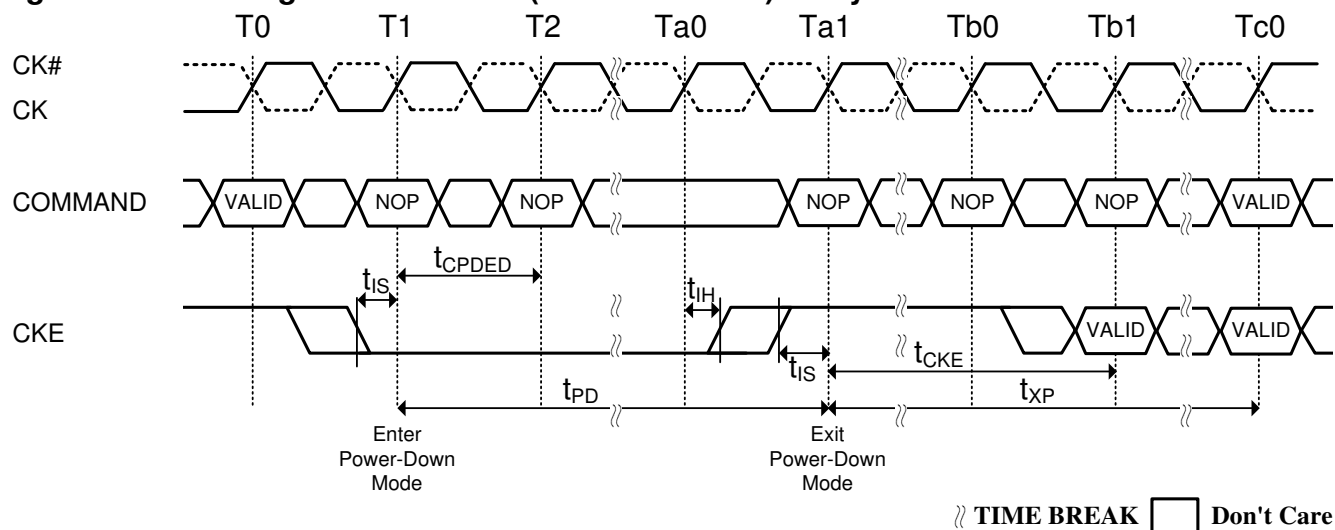
Figure 63. Precharge Power-Down (Fast Exit Mode) Entry and Exit
