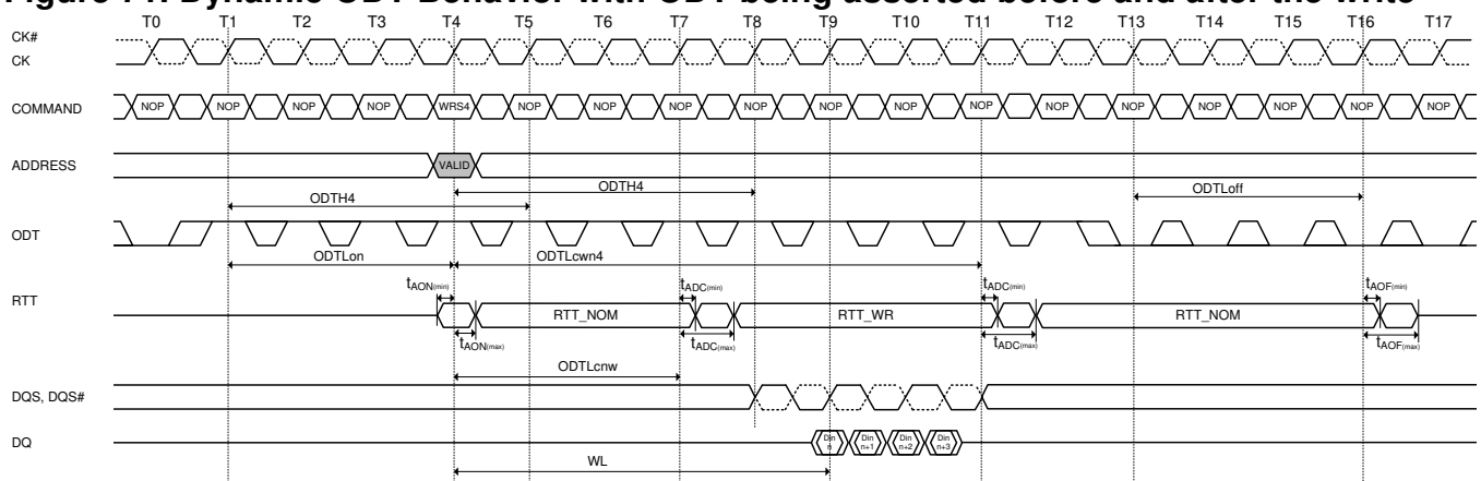
Figure 71. Dynamic ODT Behavior with ODT being asserted before and after the write
