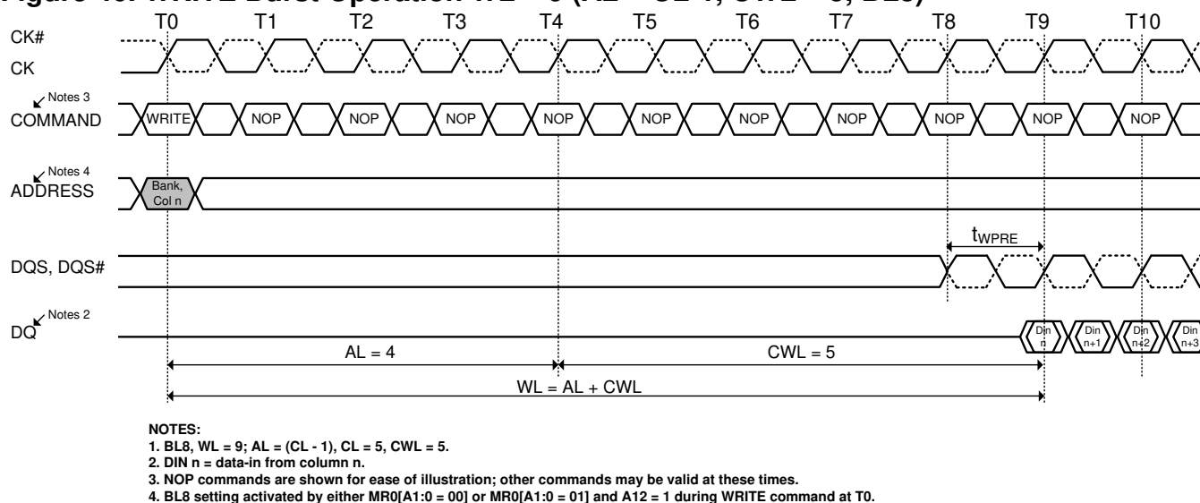
Figure 46. WRITE Burst Operation WL = 9 (AL = CL-1, CWL = 5, BL8)
