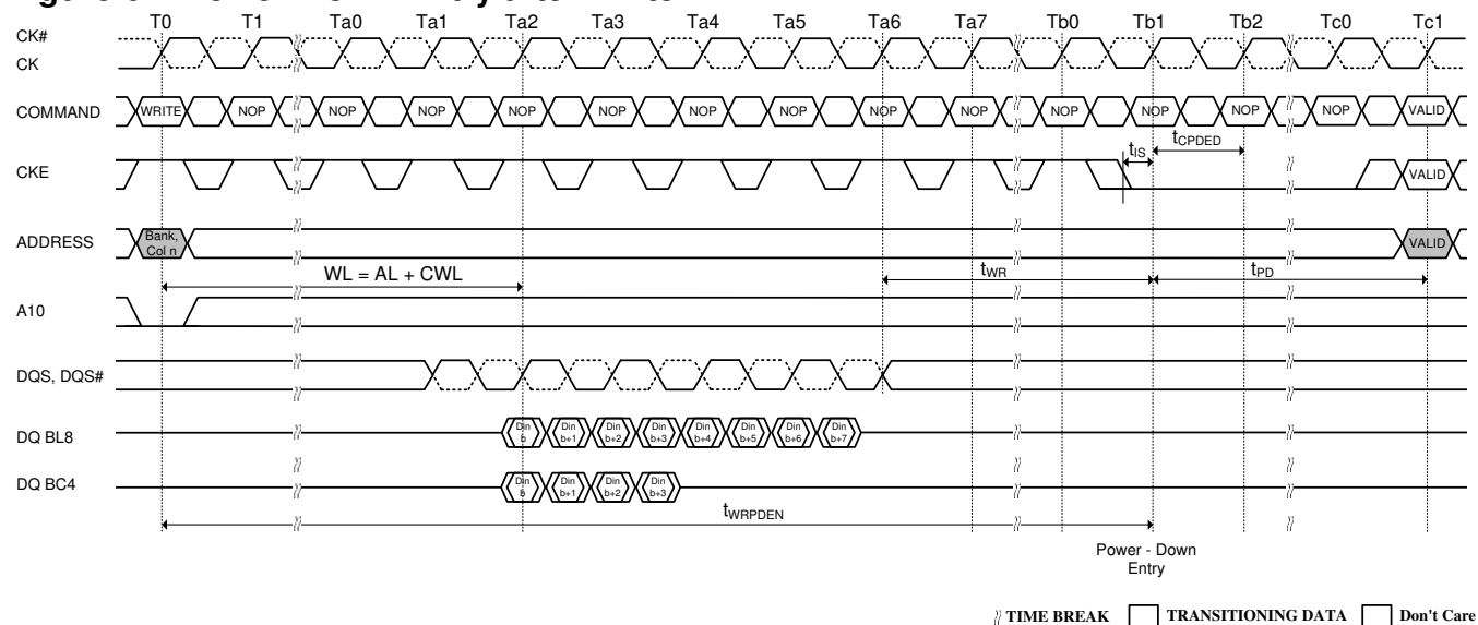
Figure 62. Power-Down Entry after Write
