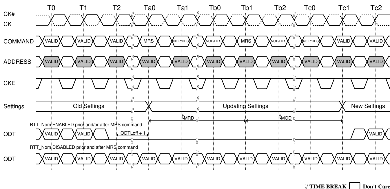
Figure 7. t_{MRD} timing
