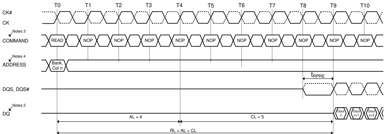
Figure 18. READ Burst Operation RL=9 (AL=4, CL=5, BL=8)
