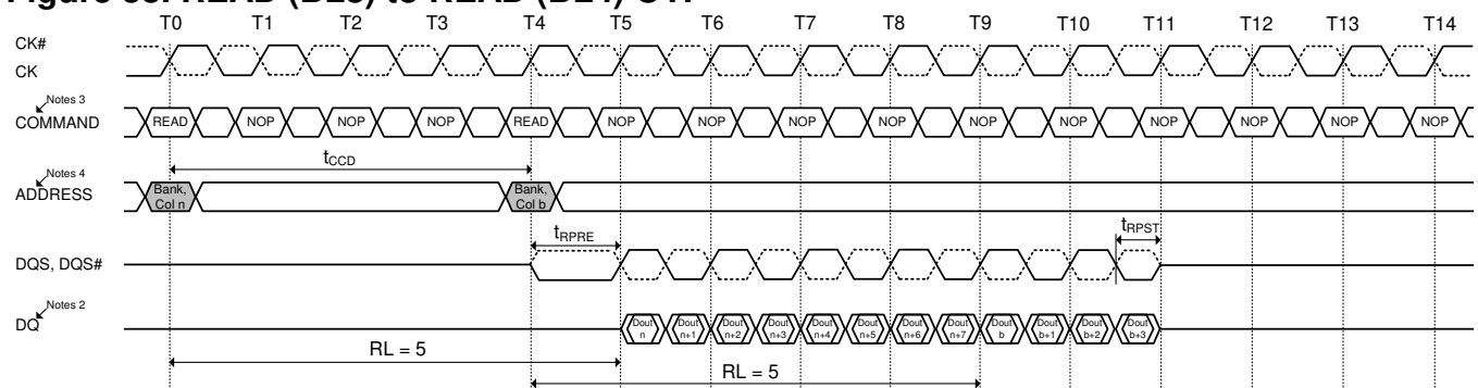
Figure 38. READ (BL8) to READ (BL4) OTF
