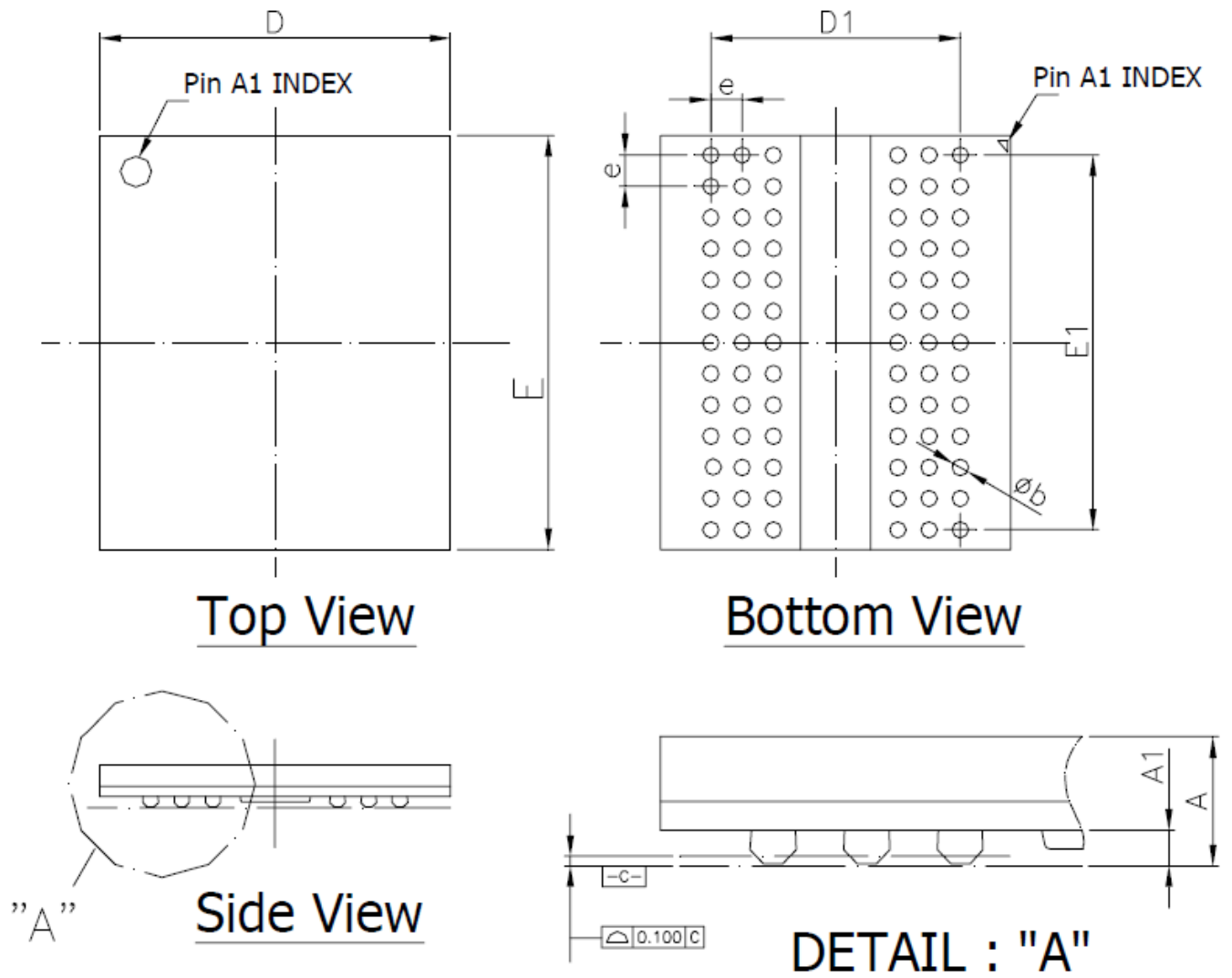
Figure 82. 78-Ball FBGA Package 9x10.6x1.2mm(max) Outline Drawing Information
