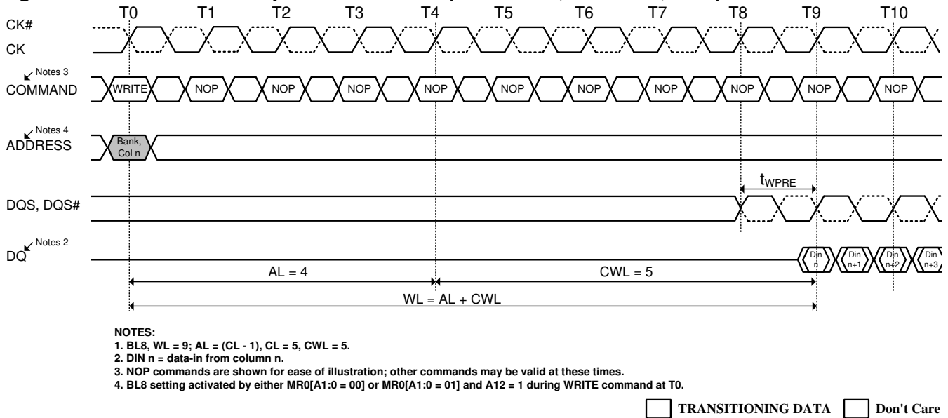
Figure 46. WRITE Burst Operation WL = 9 (AL = CL-1, CWL = 5, BL8)
