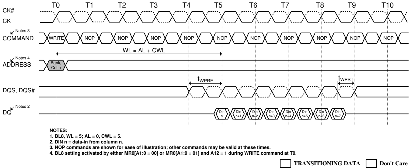
Figure 45. WRITE Burst Operation WL = 5 (AL = 0, CWL = 5, BL8)
