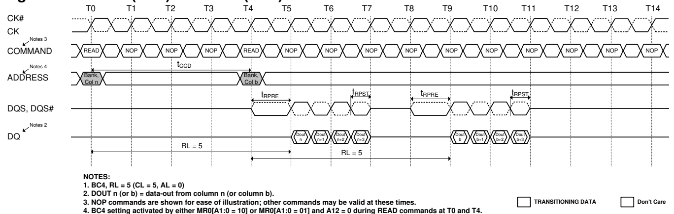
Figure 35. READ (BL4) to READ (BL4)
