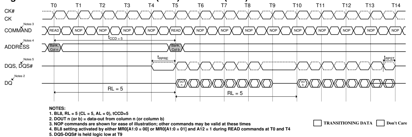
Figure 34. Nonconsecutive READ (BL8) to READ (BL8)
