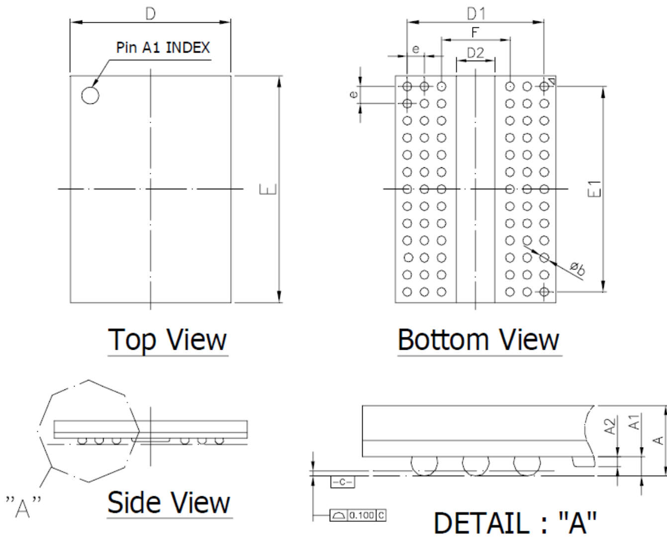
Figure 83. 78-Ball FBGA Package 7.5x10.6x1.2mm(max) Outline Drawing Information
