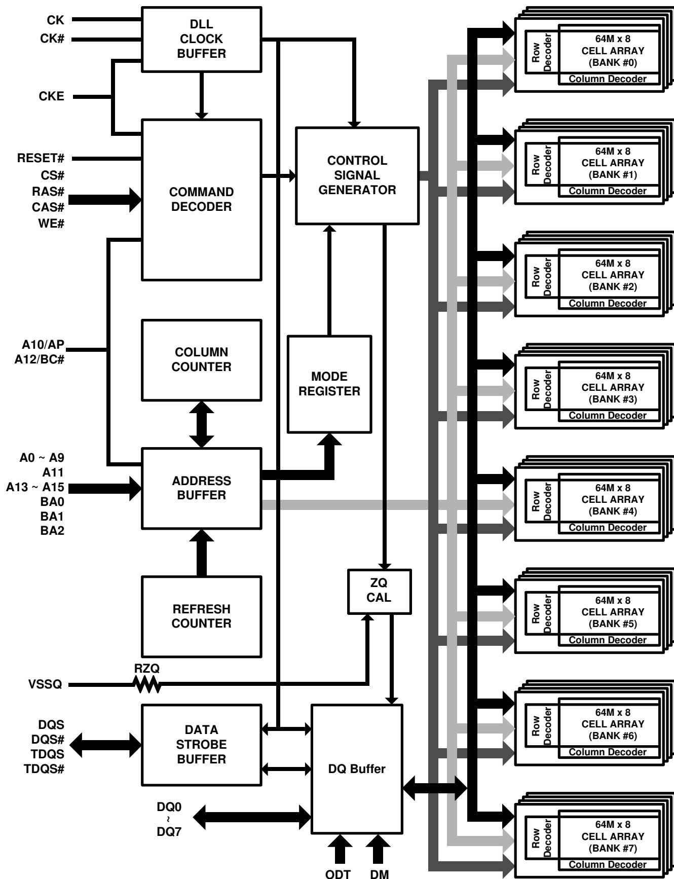
Figure 2. Block Diagram
