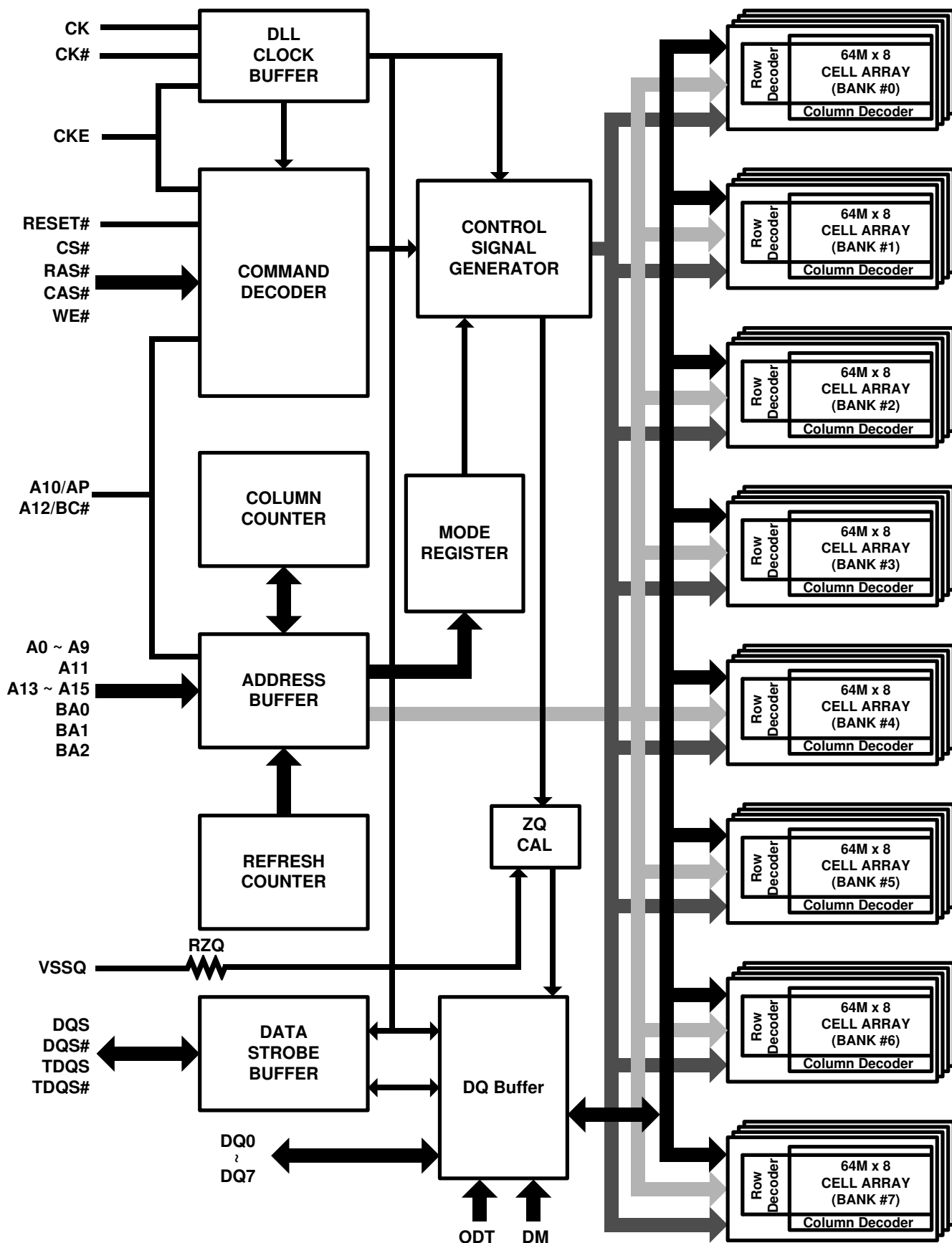
Figure 2. Block Diagram
