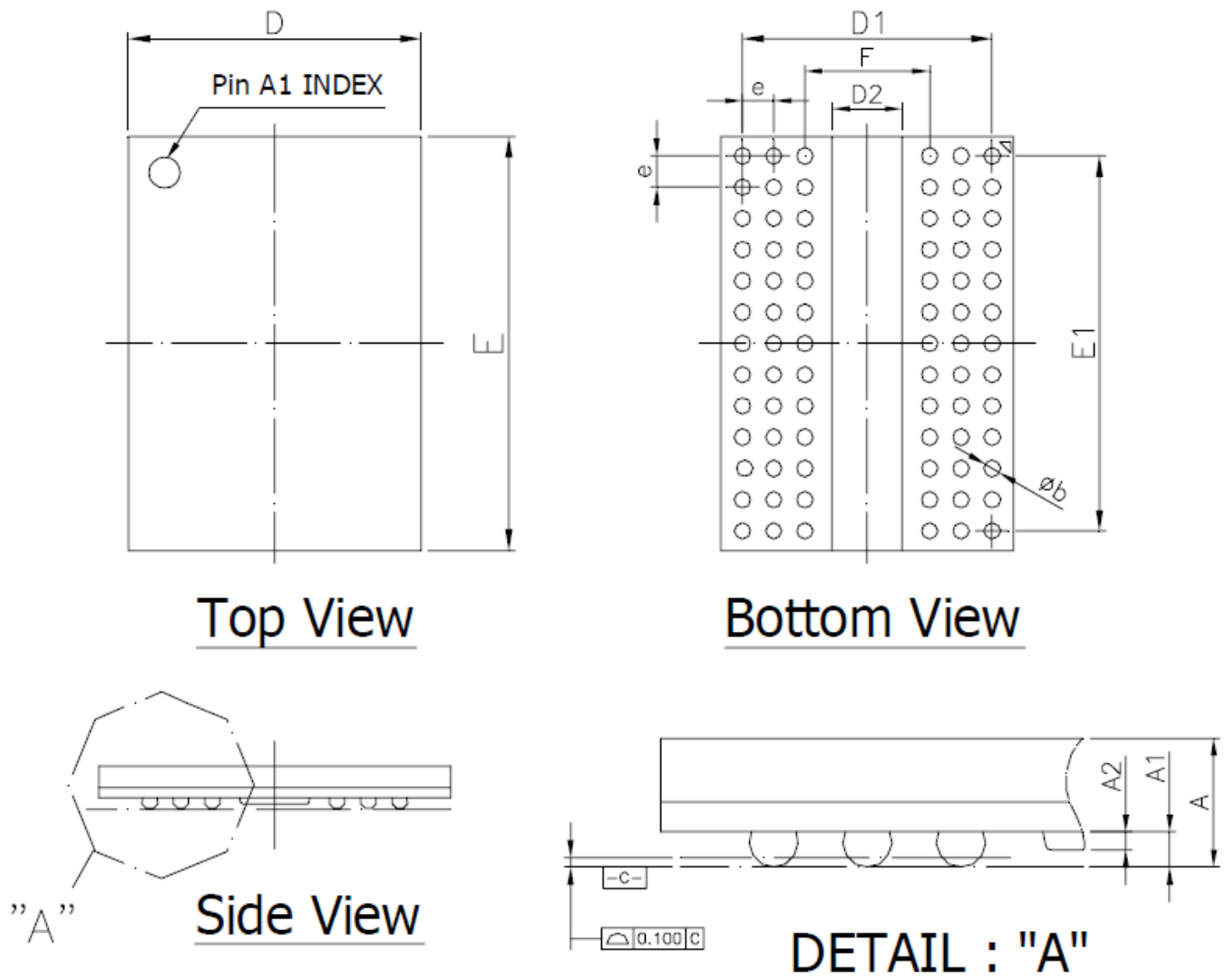
Figure 83. 78-Ball FBGA Package 7.5x10.6x1.2mm(max) Outline Drawing Information
