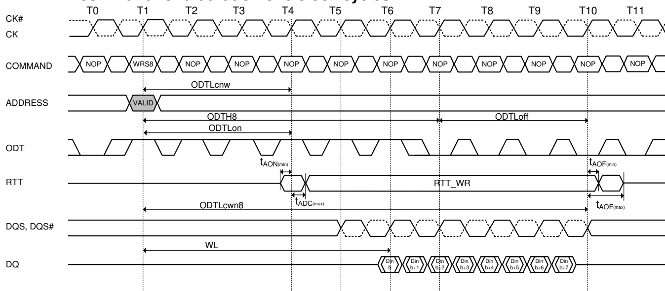
Figure 73. Dynamic ODT: Behavior with ODT pin being asserted together with write command for a duration of 6 clock cycles
