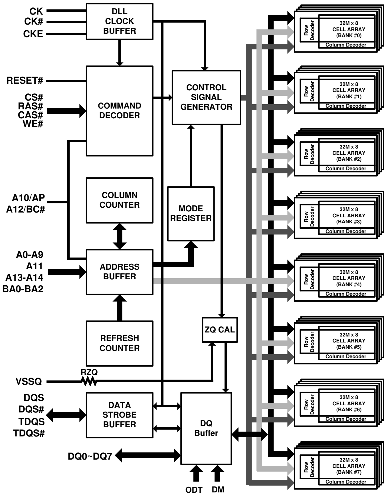
Figure 2. Block Diagram
