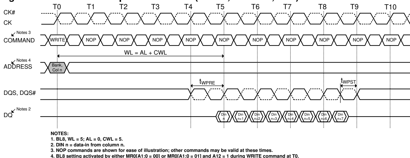
Figure 68. WRITE Burst Operation WL = 5 (AL = 0, CWL = 5, BL8)
