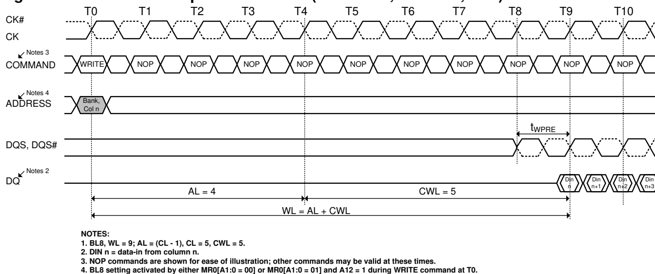
Figure 69. WRITE Burst Operation WL = 9 (AL = CL-1, CWL = 5, BL8)
