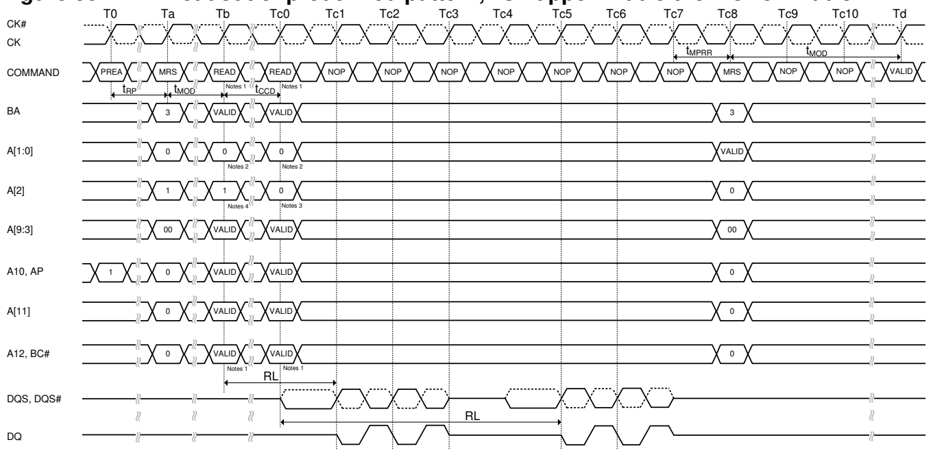
Figure 55. MPR Readout of predefined pattern, BC4 upper nibble then lower nibble
