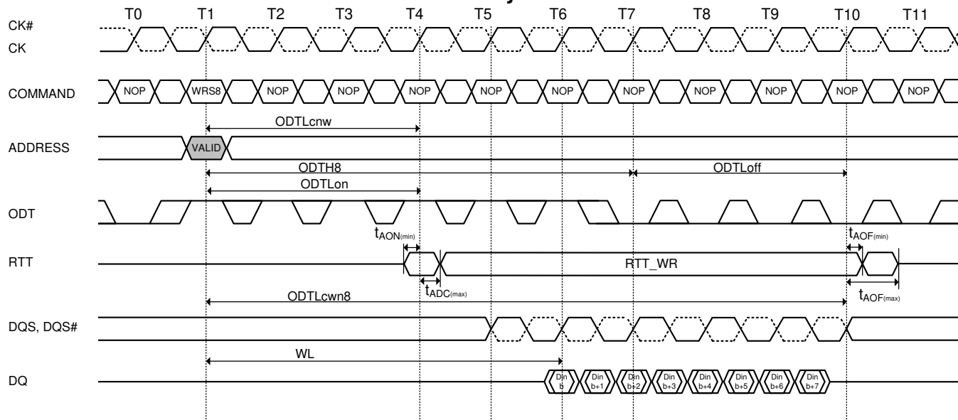
Figure 95. Dynamic ODT: Behavior with ODT pin being asserted together with write command for a duration of 6 clock cycles
