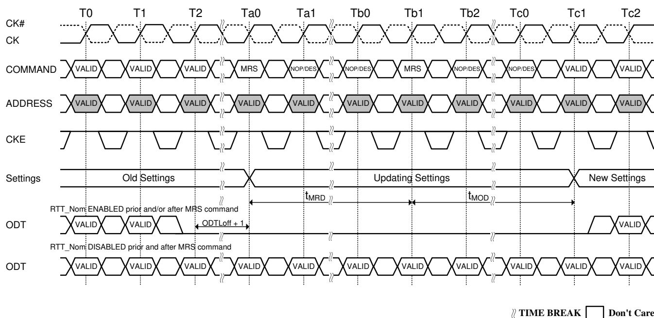
Figure 7. t_{MRD} timing
