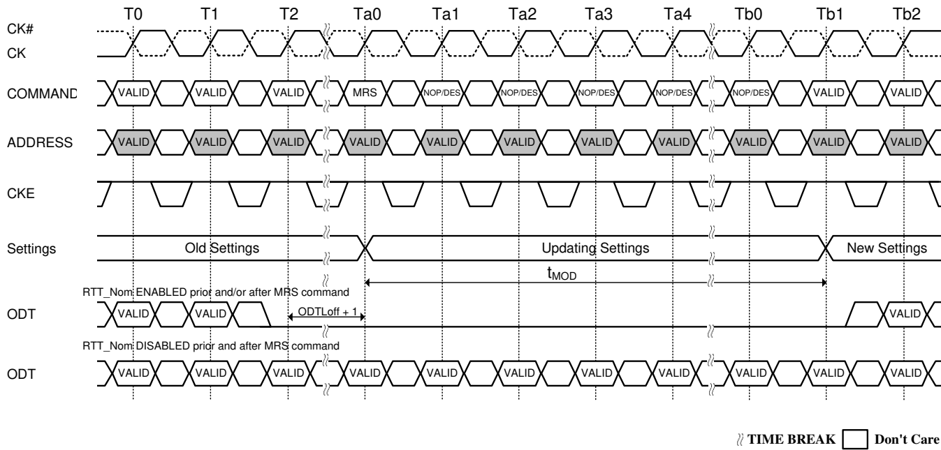
Figure 8. tMOD timing
