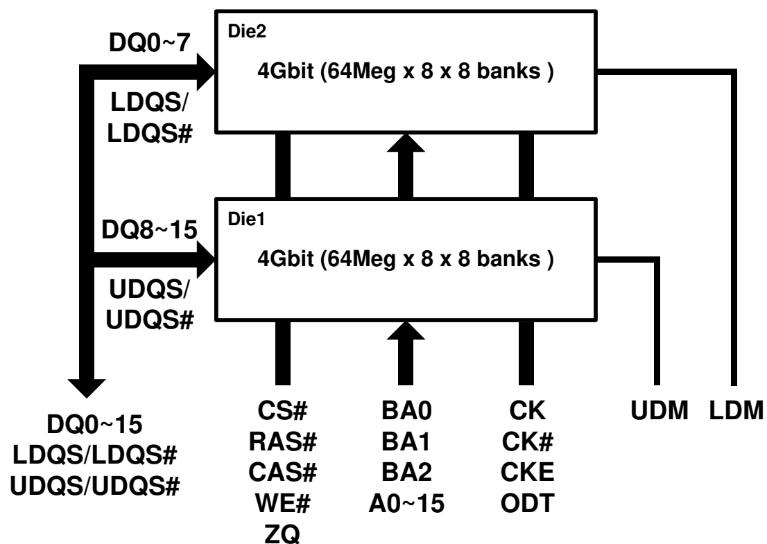
Figure 3. Stacked dice Block Diagram
