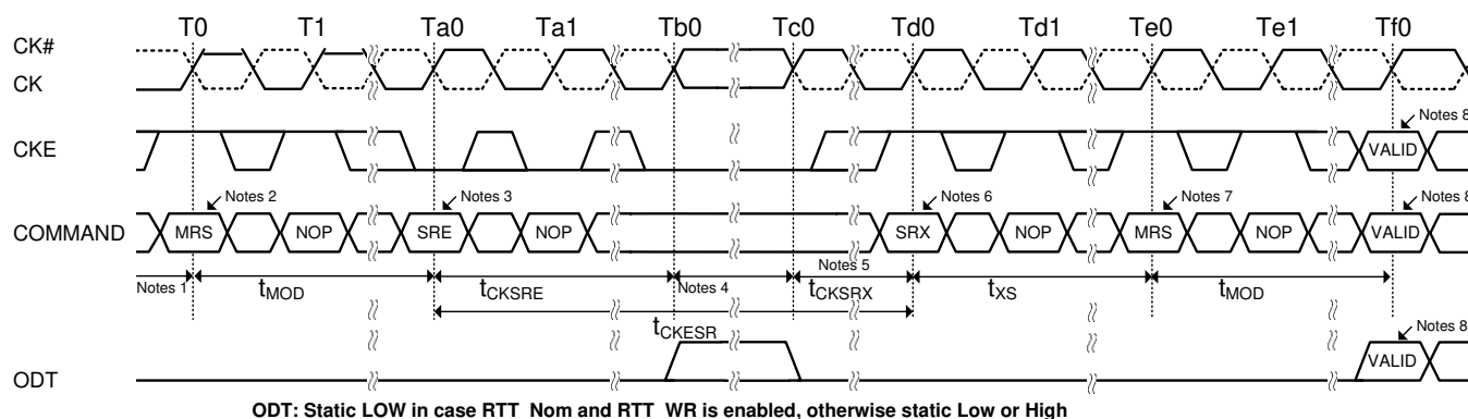
Figure 11. DLL Switch Sequence from DLL-on to DLL-off
