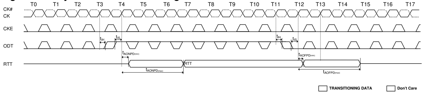
Figure 75. Asynchronous ODT Timings on DDR3 SDRAM with fast ODT transition
