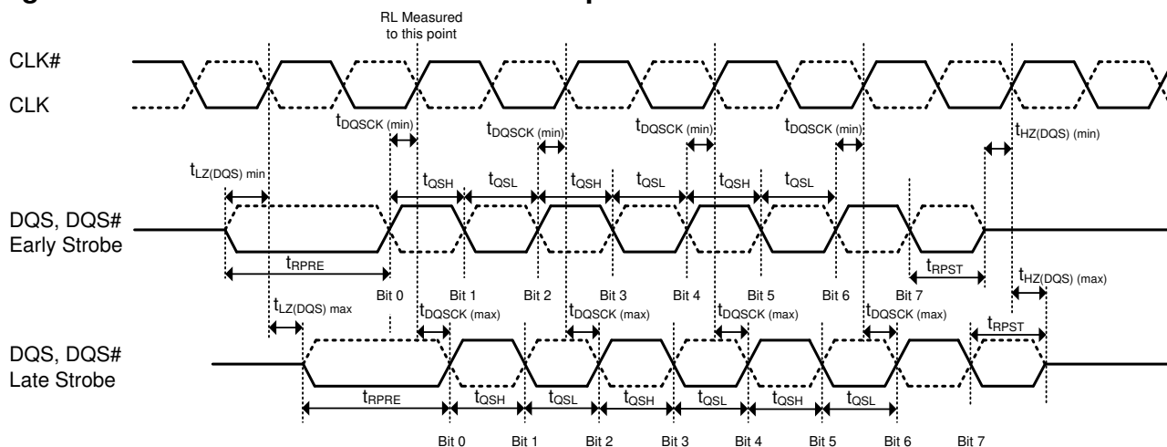
Figure 20. Clock to Data Strobe relationship
