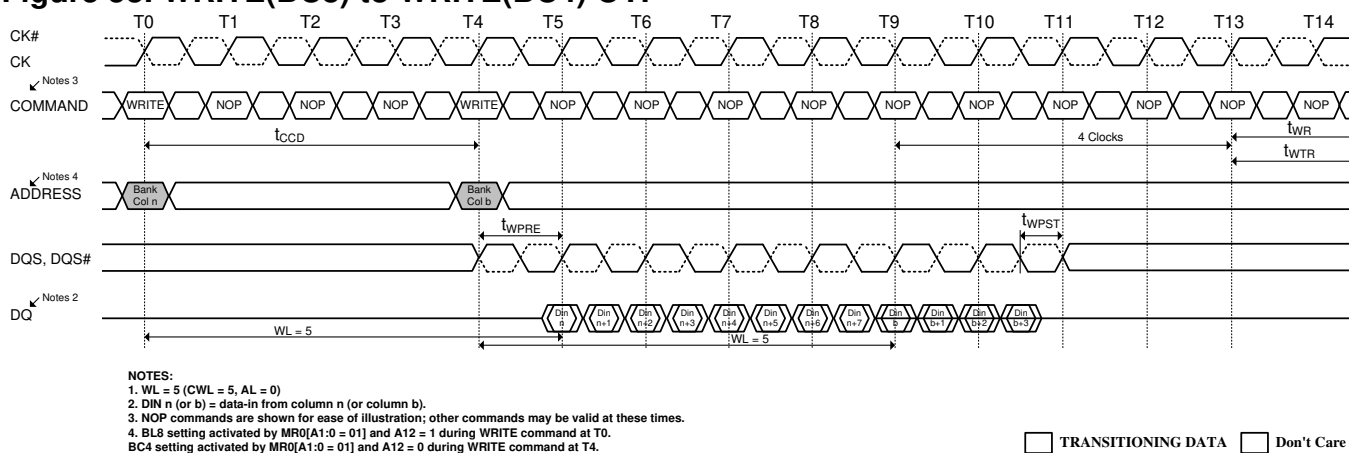
Figure 53. WRITE(BC8) to WRITE(BC4) OTF
