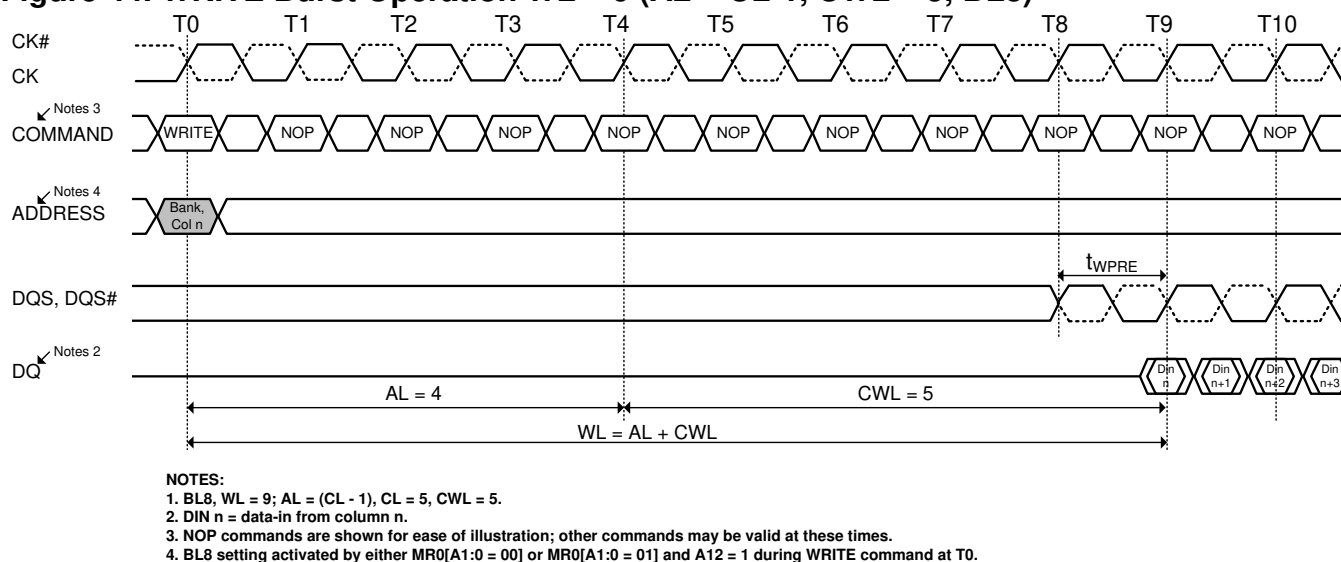
Figure 44. WRITE Burst Operation WL = 9 (AL = CL-1, CWL = 5, BL8)
