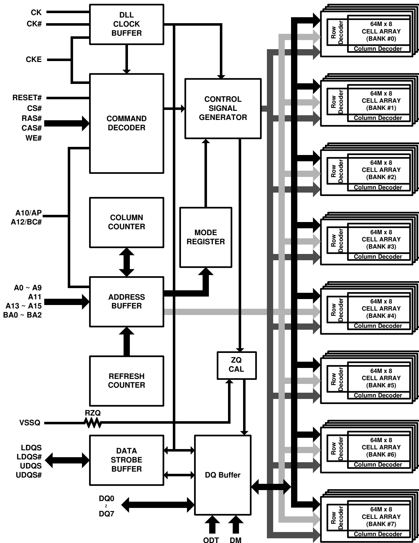
Figure 2. Block Diagram
