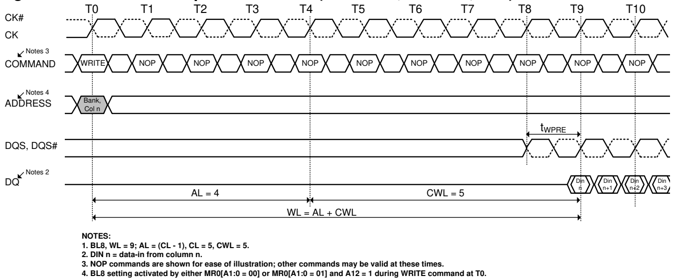
Figure 44. WRITE Burst Operation WL = 9 (AL = CL-1, CWL = 5, BL8)
