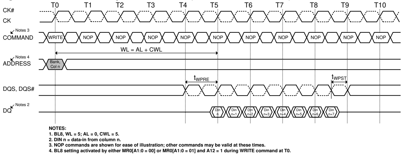
Figure 43. WRITE Burst Operation WL = 5 (AL = 0, CWL = 5, BL8)
