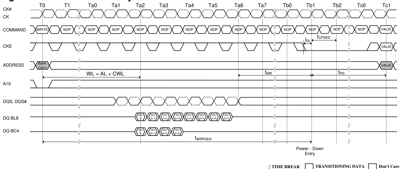
Figure 60. Power-Down Entry after Write
