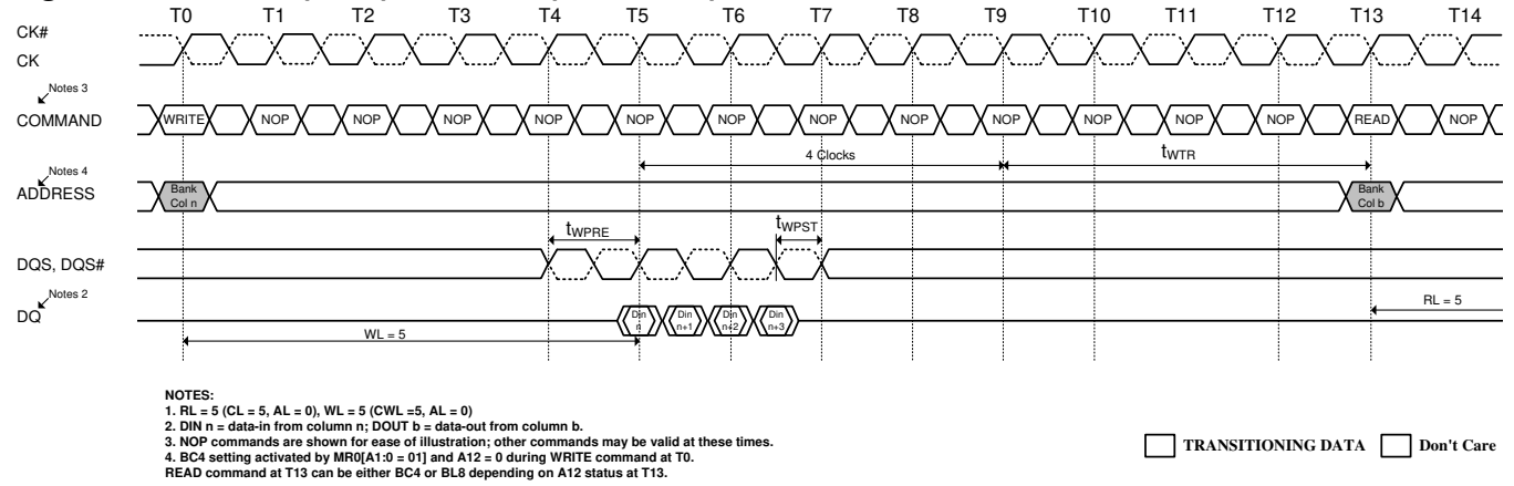
Figure 74. WRITE(BC4) to READ(BC4,BC8) OTF
