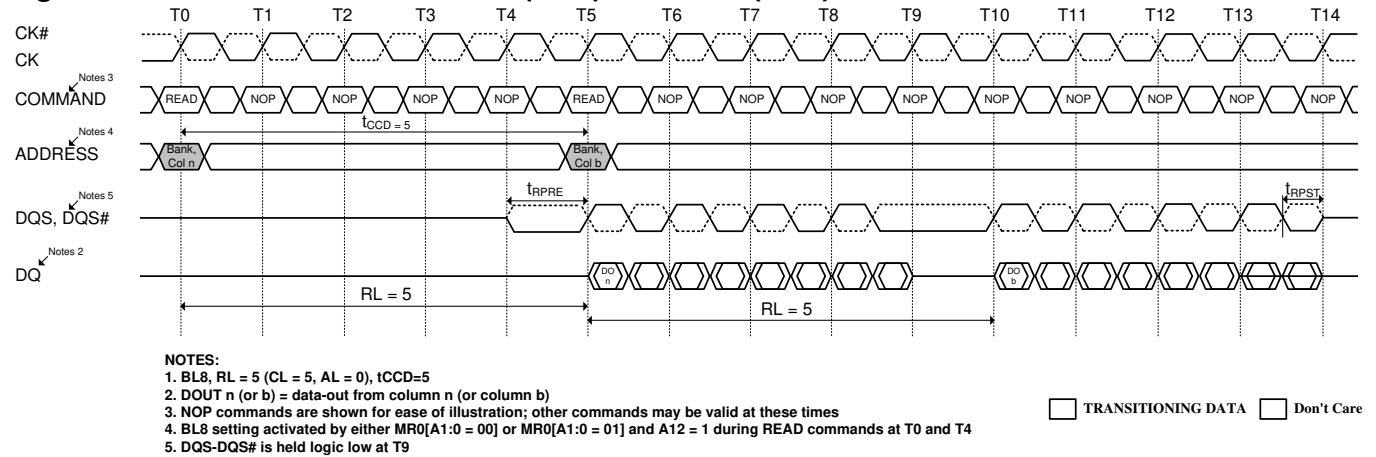
Figure 55. Nonconsecutive READ (BL8) to READ (BL8)
