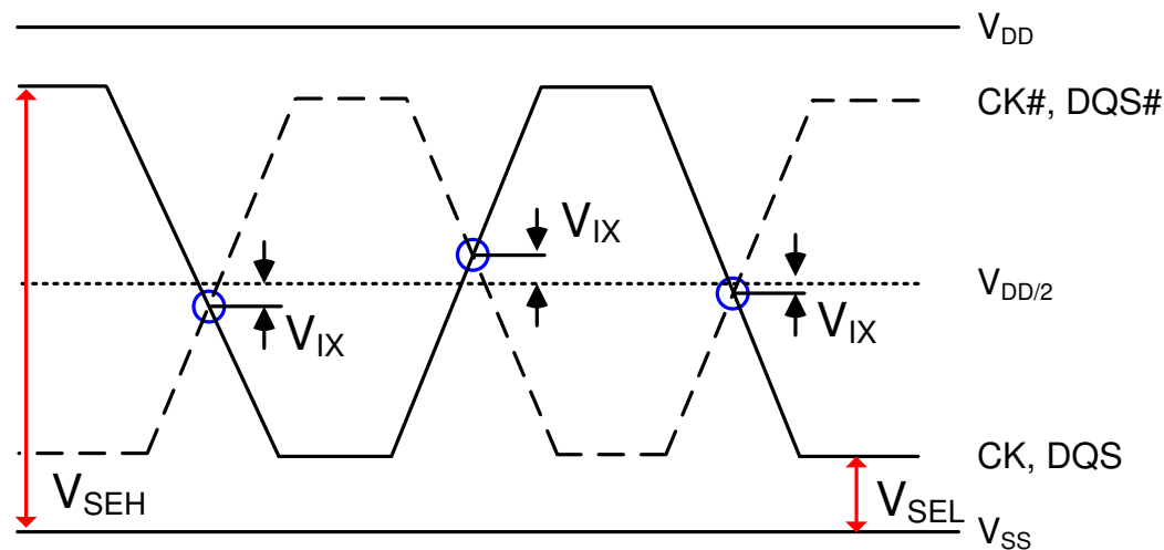
Figure 35. Vix Definition
