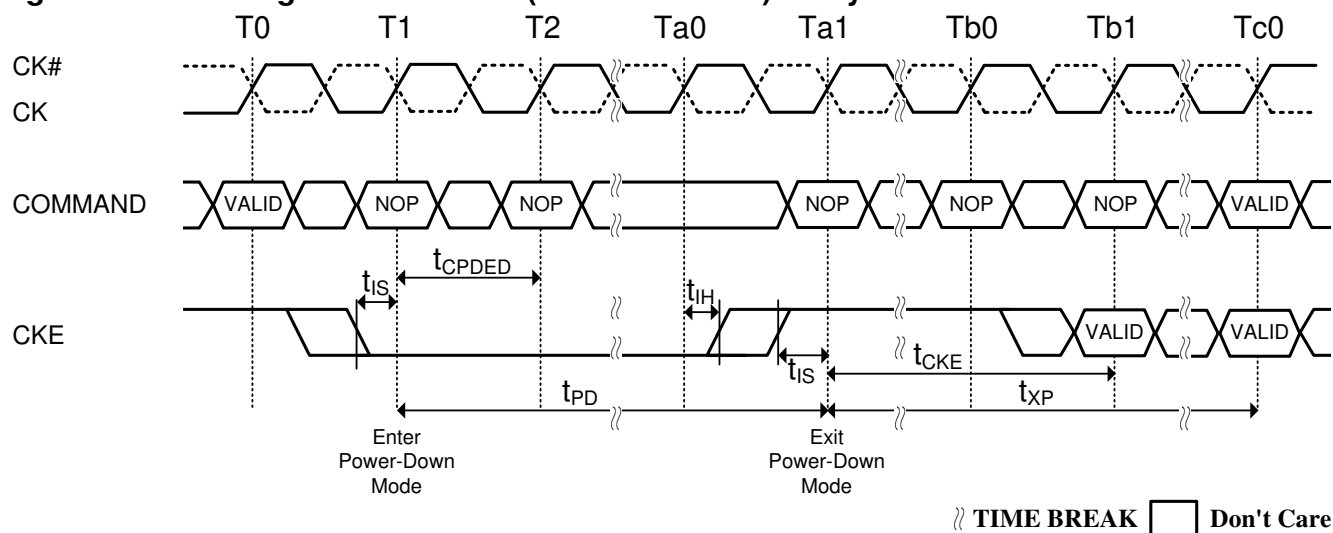
Figure 83. Precharge Power-Down (Fast Exit Mode) Entry and Exit
