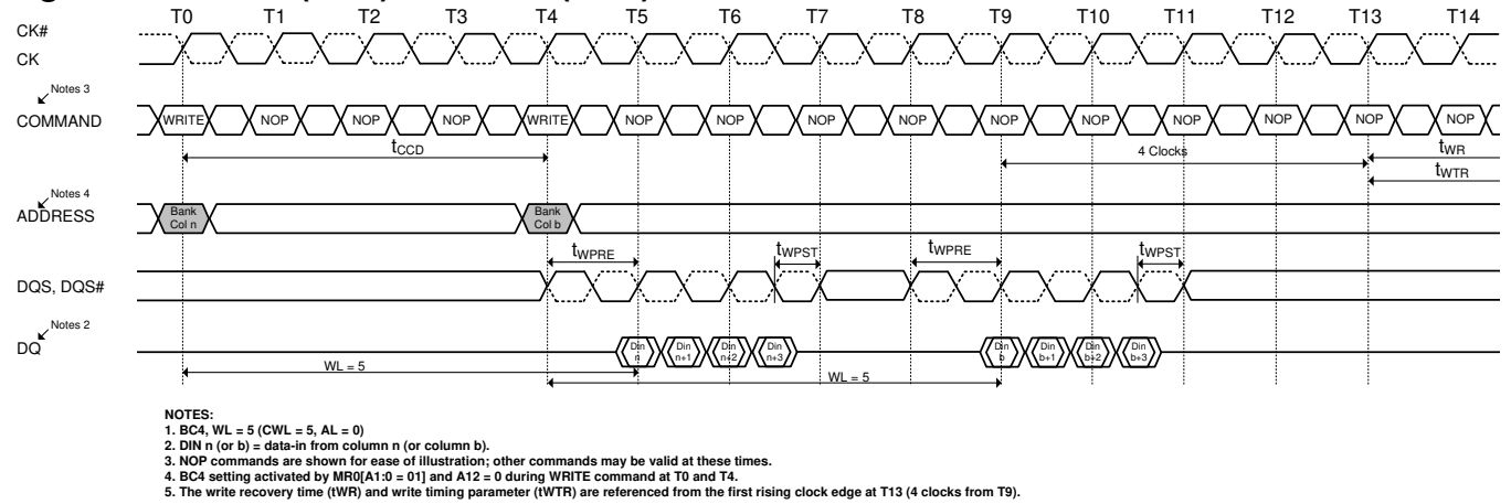
Figure 72. WRITE(BC4) to WRITE(BC4) OTF
