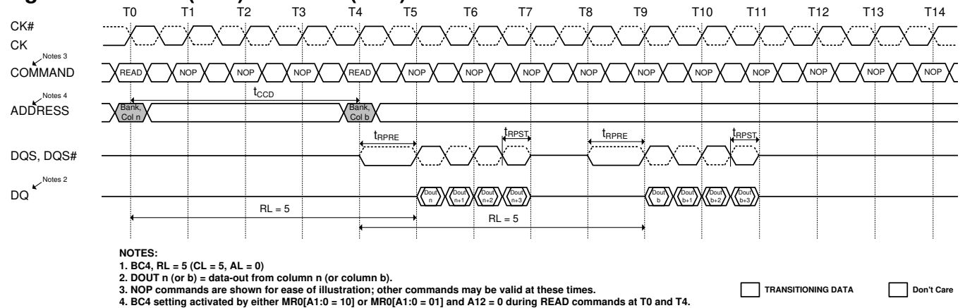
Figure 56. READ (BL4) to READ (BL4)
